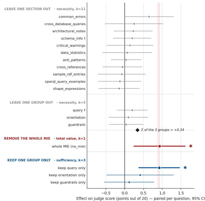
Figure 1: The redundancy arc. Eleven sections, three groups, the whole MIE, and three sufficiency conditions, all as paired per-question effects on judge score with 95% confidence intervals. Necessity is null everywhere; total value and the sufficiency of the query group are not.
