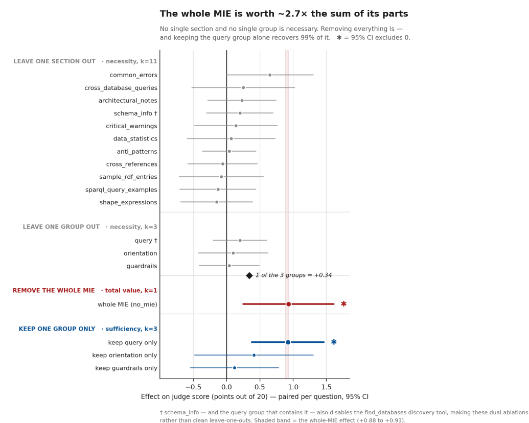
Figure 1: The redundancy arc. Eleven sections, three groups, the whole MIE, and three sufficiency conditions, all as paired per-question effects on judge score with 95% confidence intervals. Necessity is null everywhere; total value and the sufficiency of the query group are not.
