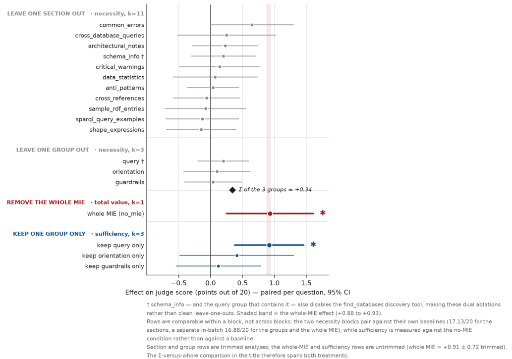
Figure 1: The redundancy arc. Eleven sections, three groups, the whole MIE, and three sufficiency conditions, all as paired per-question effects on judge score with 95% confidence intervals. Necessity is null everywhere; total value and the sufficiency of the query group are not.
