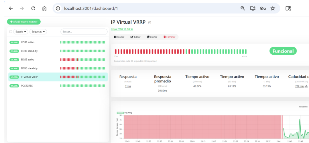
Figura 42. Etapa 1: monitor IP Virtual VRRP ( https://10.10.10.5 )
