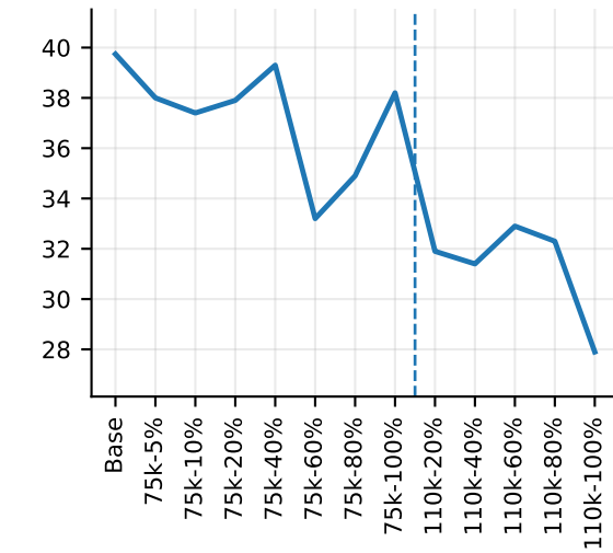
BigCodeBench-Complete
