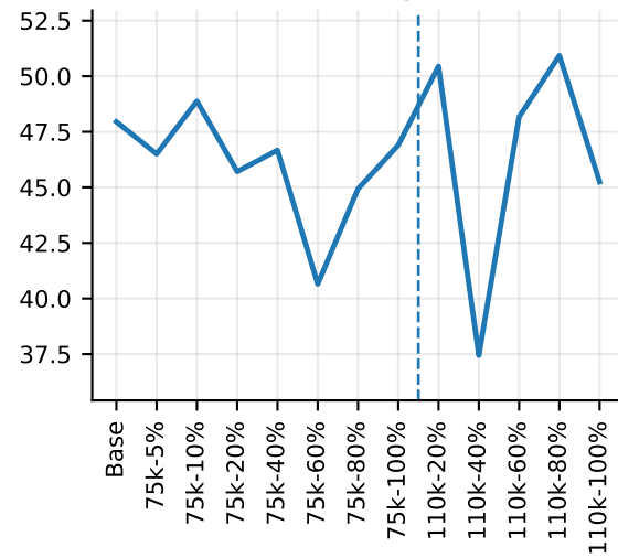
BigCodeBench-Complete
