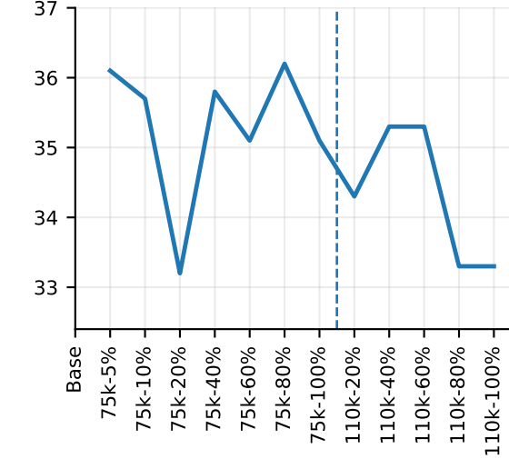
BigCodeBench-Instruct
