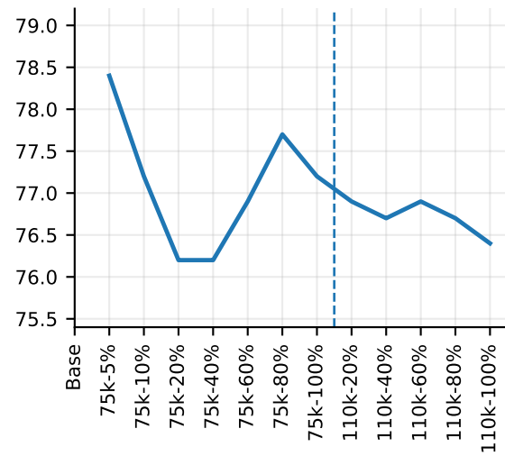
BigCodeBench-Instruct
