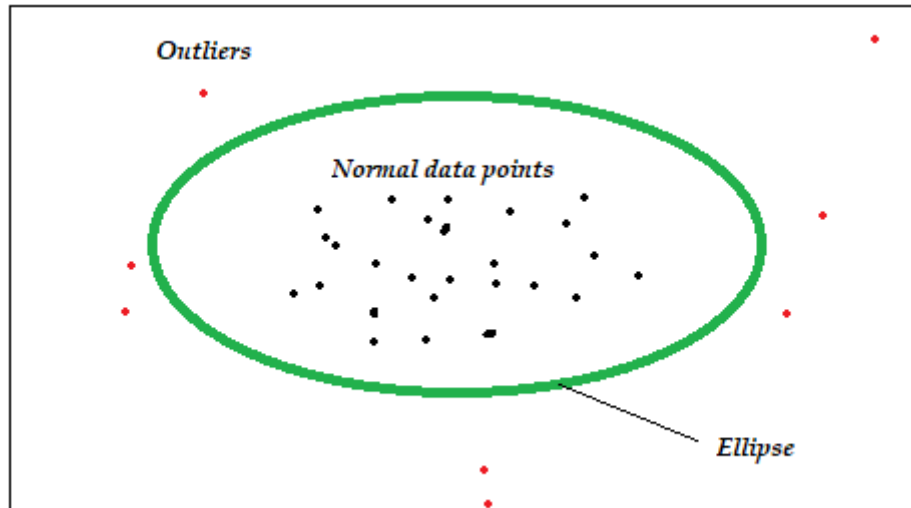
圖：在橢圓範圍外，就有可能是離群值。取自 https://medium.com/data-science/machine-learning-for-anomaly-detection-elliptic-envelope-2c90528df0a6
