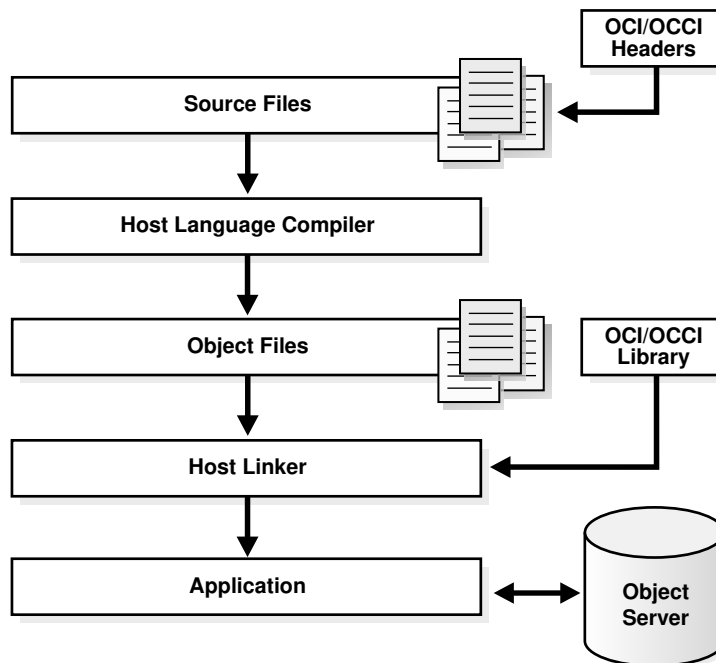
Figure 22-1 The OCI or OCCI Development Process
