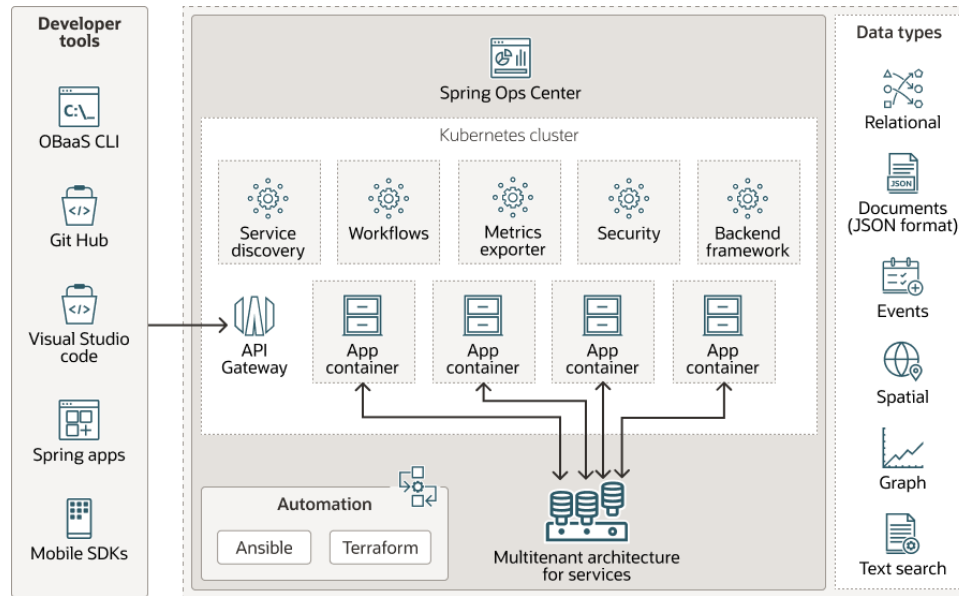
Figure 30-1 Oracle Backend for Microservices and AI (OBaaS)
