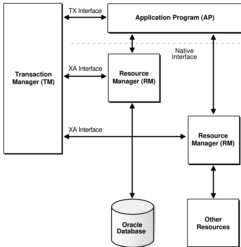
Figure 33-1 Possible DTP Model
