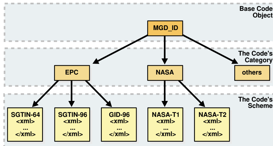
Figure 28-1 RFID Code Categories and Their Schemes
