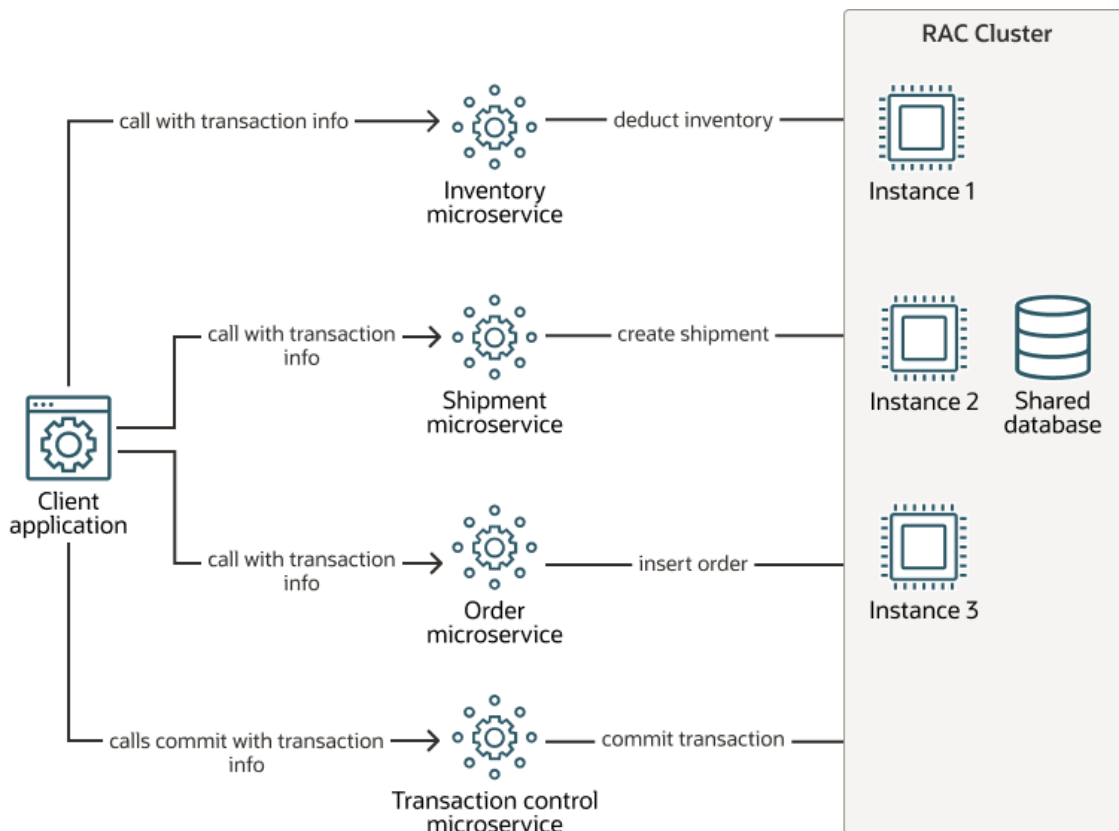
Figure 34-7 Microservices with a Single Sessionless Transaction
