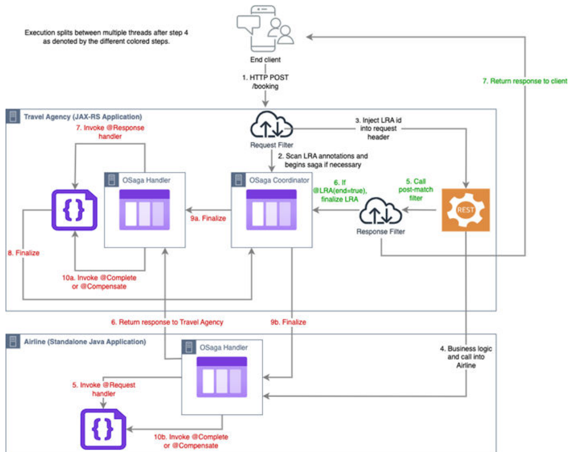
Figure 31-1 Asynchronous Flow
