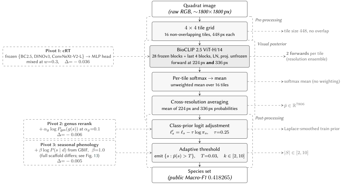
Figure 5: Inference pipeline for the headline anchor submission (solid path; public Macro F1 0.418265). Each quadrat is partitioned into a 4 \times 4 grid of 448-pixel non-overlapping tiles and forwarded through the partially fine-tuned BioCLIP 2.5 ViT-H/14 (lower 28 transformer blocks frozen; last 4 plus LN and projection unfrozen) at two inference resolutions, 224 and 336 pixels. Per-tile softmax probabilities are averaged across the 16 tiles and across the two resolutions, then class-prior logit adjustment ( \tau=0.25 ) is applied before an adaptive sigmoid threshold ( T=0.03 , k_{\min}=2 , k_{\max}=10 ) selects the output species set. Three architecture-orthogonal pivots (dashed; cRT triple-backbone classifier retraining, genus co-occurrence rerank, seasonal phenology prior) indicate where alternative configurations insert into the anchor; all three scored below the anchor on the leaderboard and are reported in Section 4.
