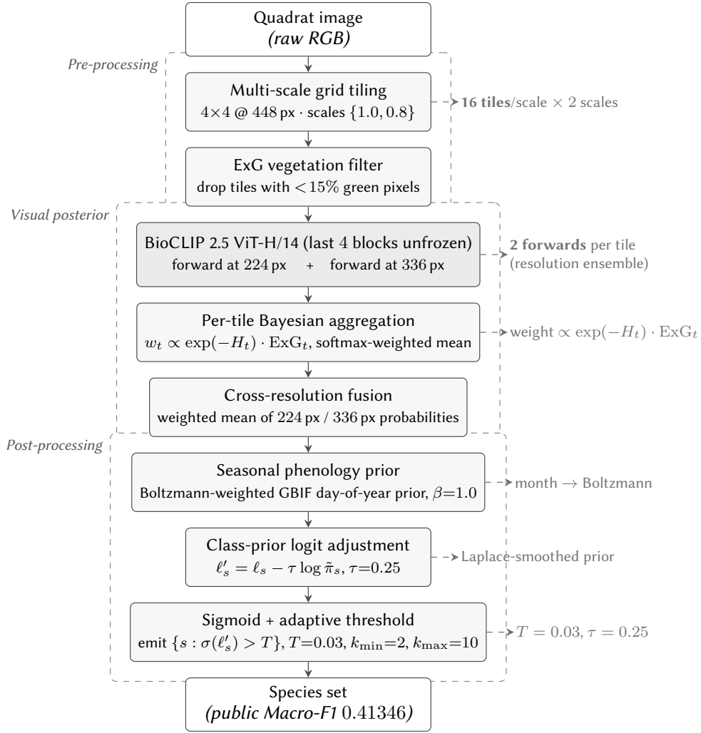
Figure 13: Inference pipeline for the seasonal phenology submission (Pivot 3, public Macro F1 0.41346). Each quadrat is processed at two grid scales (1.0 and 0.8); tiles are screened by an Excess Green (ExG) vegetation filter; the surviving tiles are forwarded through the partially fine-tuned BioCLIP 2.5 ViT-H/14 at two inference resolutions (224 and 336 pixels). Per-tile probabilities are pooled by entropy-weighted Bayesian aggregation, w_t \propto \exp(-H_t) \cdot \text{ExG}_t , and the two resolutions are then averaged. A Boltzmann-weighted seasonal phenology prior over the GBIF day-of-year histogram is added in log space at \beta=1.0 , followed by class-prior logit adjustment ( \tau=0.25 ) and adaptive sigmoid threshold selection ( T=0.03 , k_{\min}=2 , k_{\max}=10 ). The pipeline differs from the anchor (Figure 5) in its multi-scale tiling, ExG screening, and entropy-weighted aggregation; the phenology log-prior is the additional term unique to this submission.
