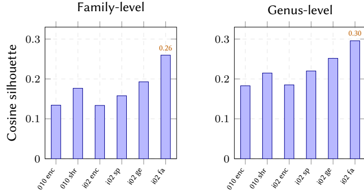
Figure 11: Taxonomic structure of each head representation on the family stratified 4,000-image samples: cosine silhouette at the family and genus levels. Within each experiment the trained MLP increases structure over its own raw encoder feature; within i002 the family and genus MLPs are the most structured (family level silhouette 0.26 for the family MLP versus 0.16 for the species MLP). Magnitudes are comparable only within an experiment, not across, because the two experiments use different validation samples.
