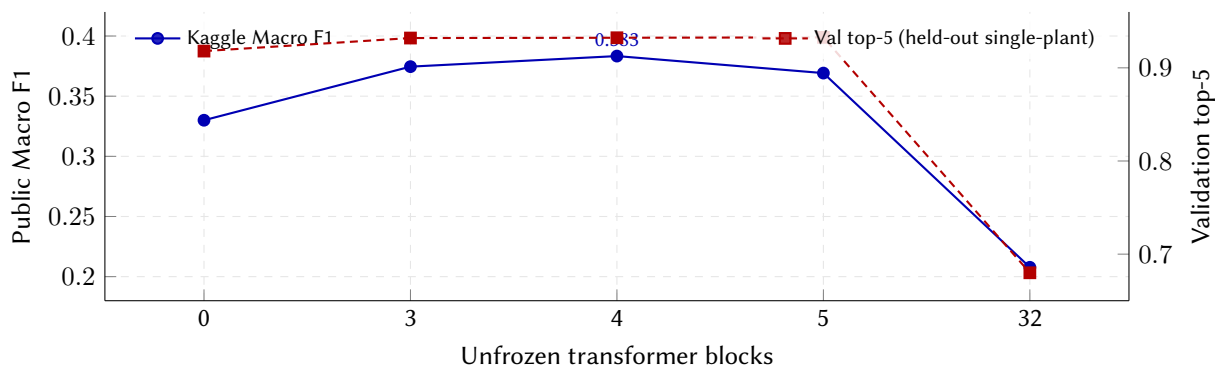
Figure 6: Unfrozen-blocks sweep visualised with both metrics. Held-out validation top-5 (dashed, right axis) rises monotonically with capacity from n=0 to n=5 , but Kaggle Macro F1 (solid, left axis) peaks sharply at n=4 and collapses at full fine-tune ( n=32 ). The disagreement between the two curves is examined in §5.1: validation accuracy on the single-plant distribution does not predict multi-species quadrat Macro F1.
