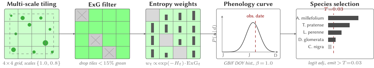
Figure 15: Data flowing through the seasonal phenology submission, stage by stage. Multi-scale tiling: the input quadrat is partitioned into a 4 \times 4 grid at the native scale (solid lines) and re-partitioned at scale 0.8 (dashed inner rectangle), giving two tile sets. ExG filter: each tile's Excess Green index \text{ExG}_t = 2G_t - R_t - B_t is computed and tiles with fewer than 15% green pixels are dropped (greyed out with a cross). Entropy weights: the surviving tiles are weighted by w_t \propto \exp(-H_t) \cdot \text{ExG}_t , where bar height encodes the weight; confident, vegetation-rich tiles dominate the softmax-weighted mean. Phenology curve: the per-species observability density P(s | d) , smoothed from the GBIF month-of-observation histogram, is multiplied into the posterior in log space at \beta=1.0 , where the dashed red line marks the quadrat's observation date d . Species selection: after class-prior logit adjustment, species whose probability exceeds T=0.03 are emitted; the bottom bar (greyed) falls below threshold and is rejected.
