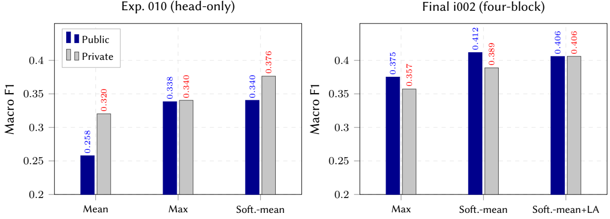
Figure 8: Two-stage tile-aggregation comparison (public and private Macro F1). The left panel is the earlier experiment 010 head-only checkpoint at matched tile geometry ( grid_4x4 , tile size 448, overlap 0.5), where plain mean was explored and found weakest, so it was dropped. The right panel is the final i002 four-block checkpoint ( grid_4x4 , no overlap, 224 pixels), where the submitted comparison was max against softmax-mean only; plain mean is intentionally absent from this panel because it was not re-submitted on this checkpoint. Softmax-mean improves on max on both splits, and softmax-mean with logit adjustment ( \tau=0.25 ) is the most robust on the private split. Each bar is the best-public or best-private selection for that mode.
