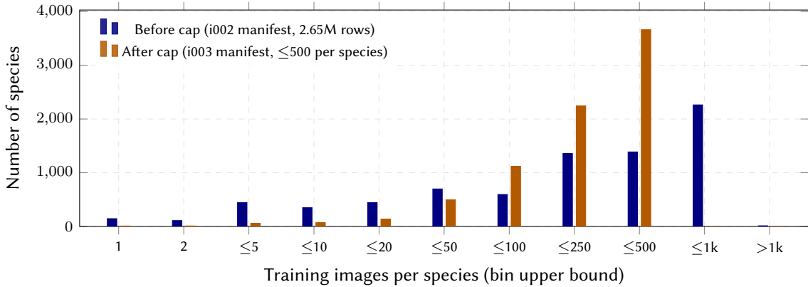
Figure 12: Species count per training-image bin, before and after the i003 per-species cap at 500. The cap collapses the two heaviest bins ( \leq 1k and > 1k ) into the \leq 500 bin and lifts middle bins, but does not move species out of the long tail (left bins). This flatter distribution hurt the public Macro F1.
