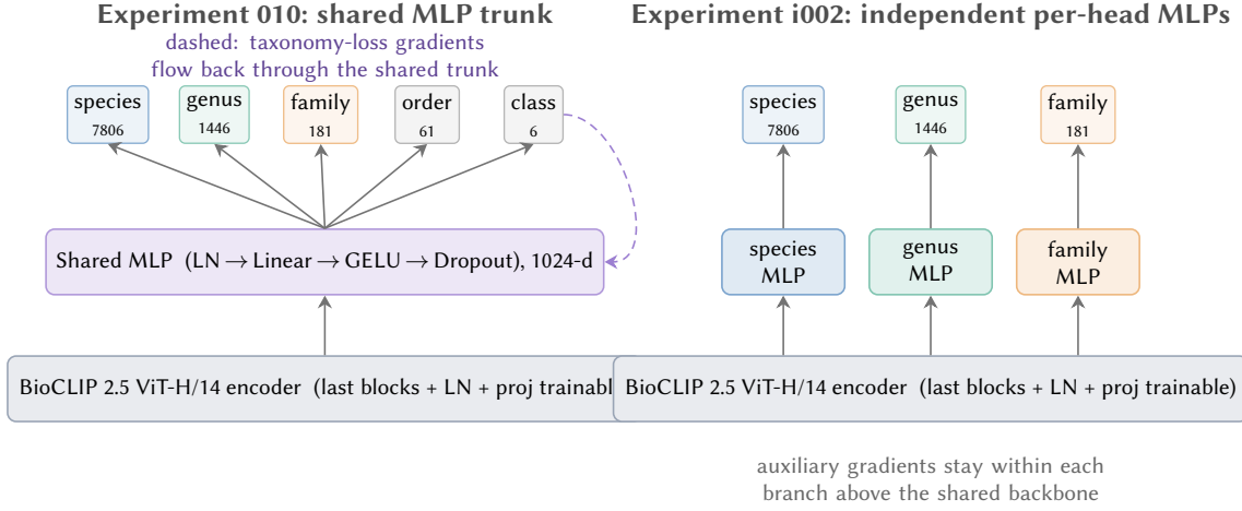
Figure 4: Head designs of the two supervised fine-tunes. Experiment 010 (left) uses a single shared MLP (layer normalisation, a linear projection of the 1,024-d embedding, GELU, and dropout) whose hidden vector feeds five linear heads (species/genus/family/order/class); the auxiliary taxonomy losses back propagate through the shared trunk. Experiment i002 (right) uses three independent per head MLPs (species/genus/family), so the auxiliary gradients do not pass through the species MLP. Both share the partially unfrozen BioCLIP 2.5 backbone (last blocks plus the final layer norm and projection). The diagram shows the design difference only: the two experiments are not a controlled ablation, since they also differ in training data, schedule, unfrozen blocks, and head count.
