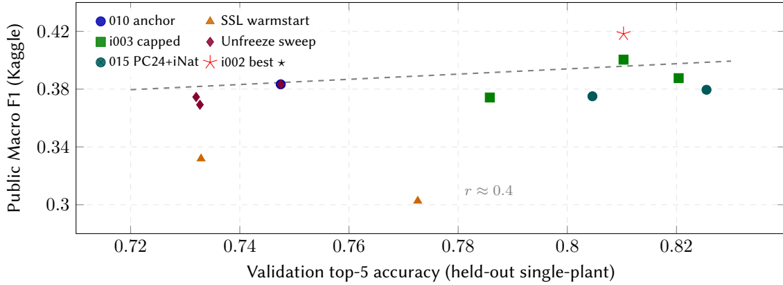
Figure 10: Validation top-5 accuracy on the held-out single-plant split versus public Macro F1 on the multi-species quadrat leaderboard, across our twelve strongest runs. The headline anchor (★, i002 last-four-blocks 224+336+LA ensemble) does not sit at the maximum validation point; the i003 capped checkpoints (green squares) and the 015 PC24+iNat mix (teal) reach higher validation accuracy but lower leaderboard score. The dashed line indicates the weak monotone trend ( r \approx 0.4 ).
