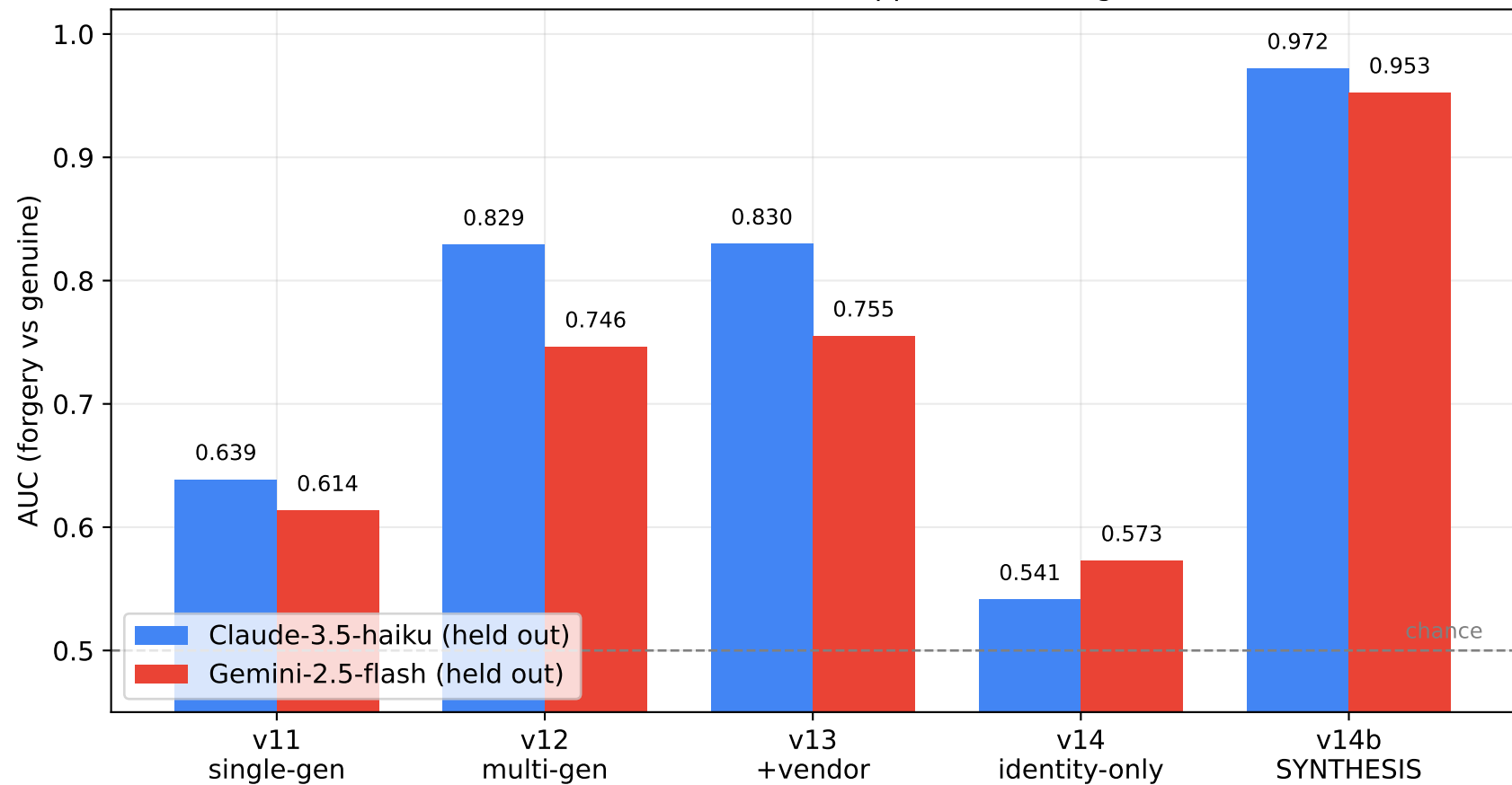
Cross-generator generalization: detecting forgeries from UNSEEN models (Claude + Gemini never appear in training)
