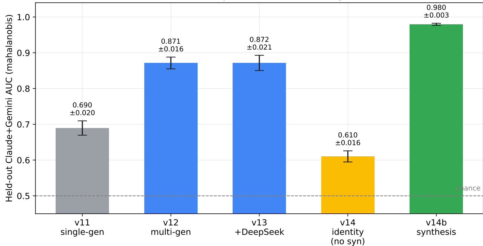
Cross-generator detection across the version lineage (mean \pm std over 5 probe draws; held-out generators)
