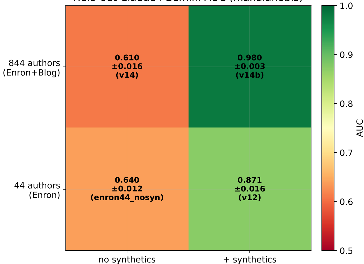
Identity \times synthetic 2 \times 2 Held-out Claude+Gemini AUC (mahalanobis)
