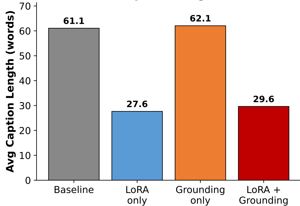
Caption Length
