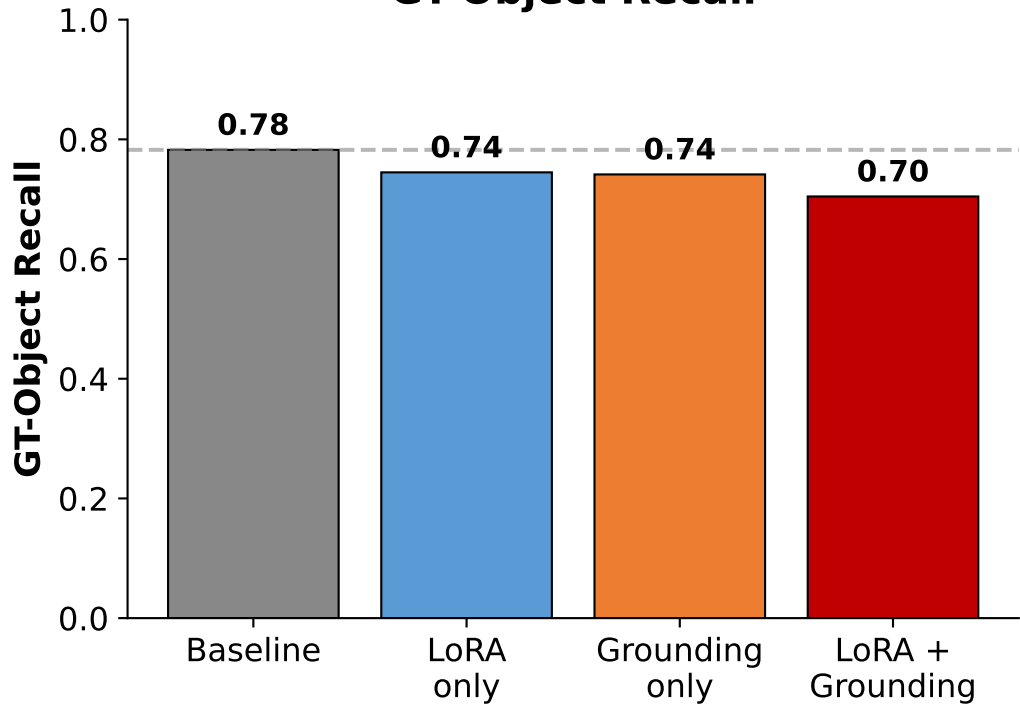
GT-Object Recall
