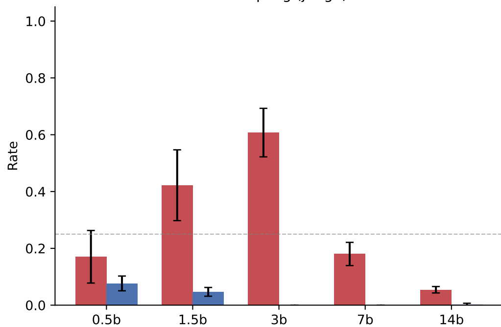
Decoupling (judge)
