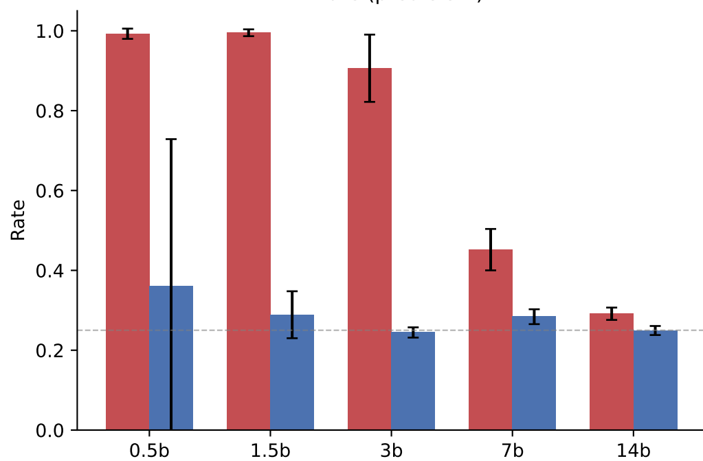
Decoupling (judge)
