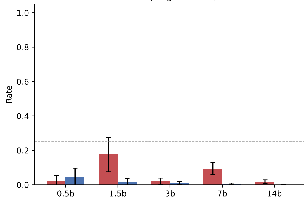
Decoupling (numeric)
