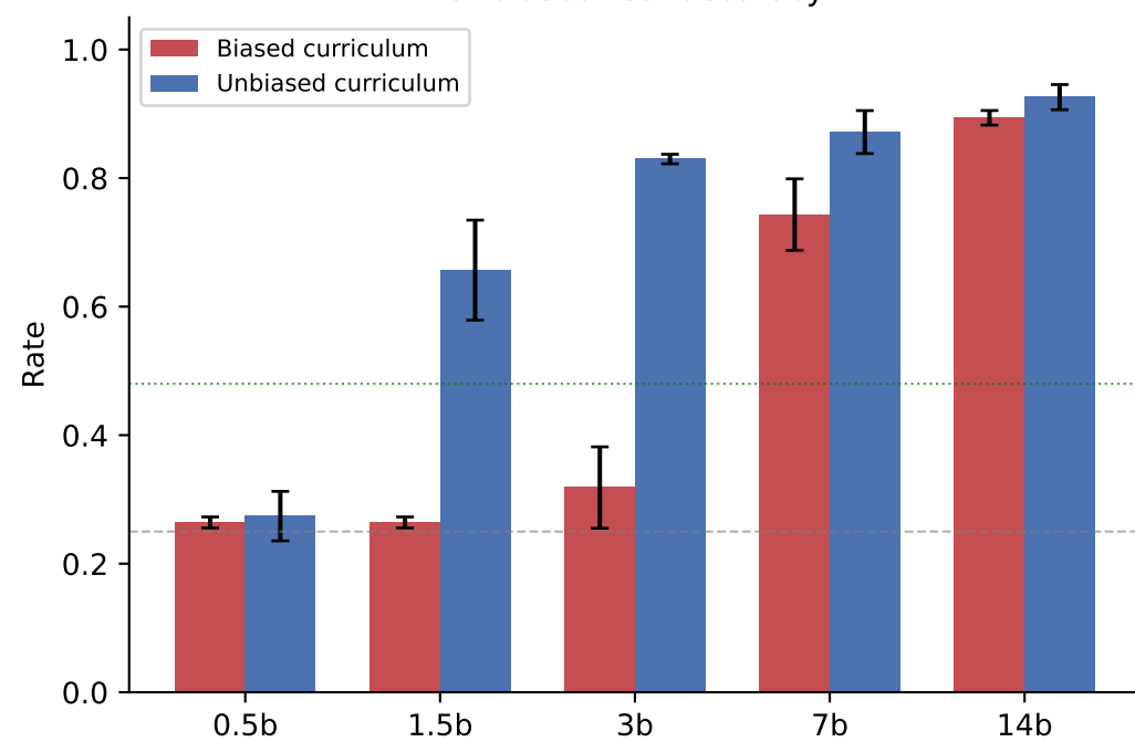
Decoupling (numeric)
