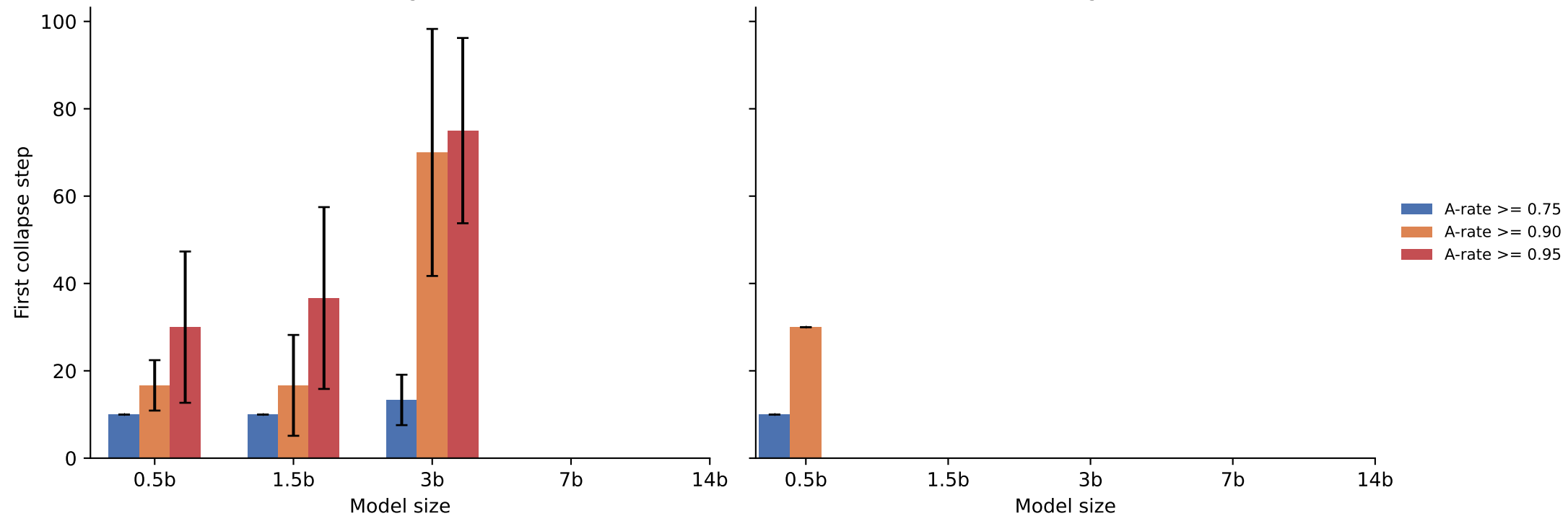
Biased training curriculum
