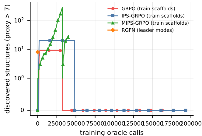
(b) discovery during training
