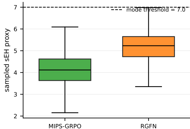
(a) final-policy reward distribution
