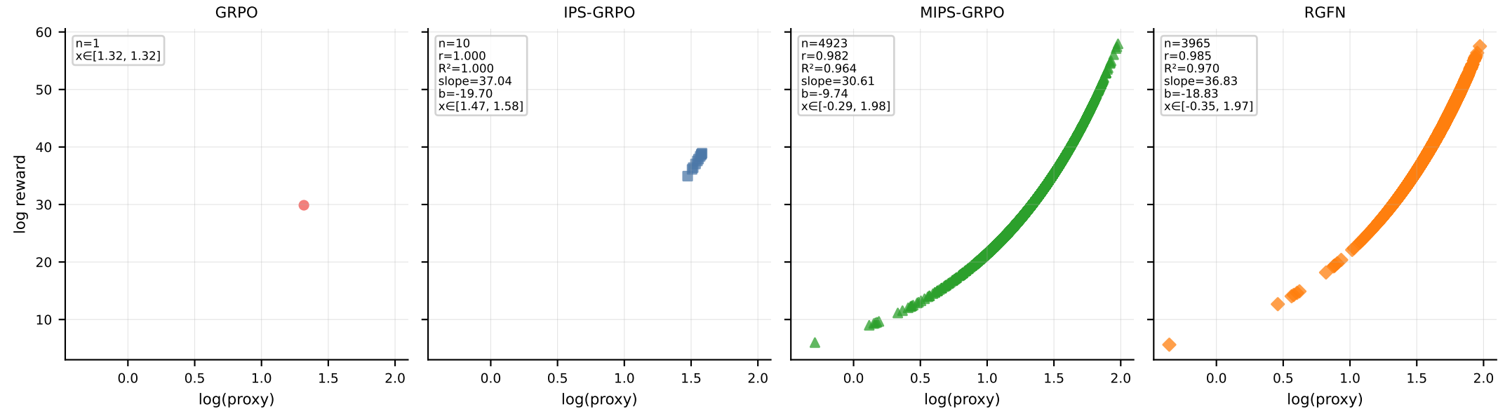
Supplementary: unique-terminal log reward vs log proxy
