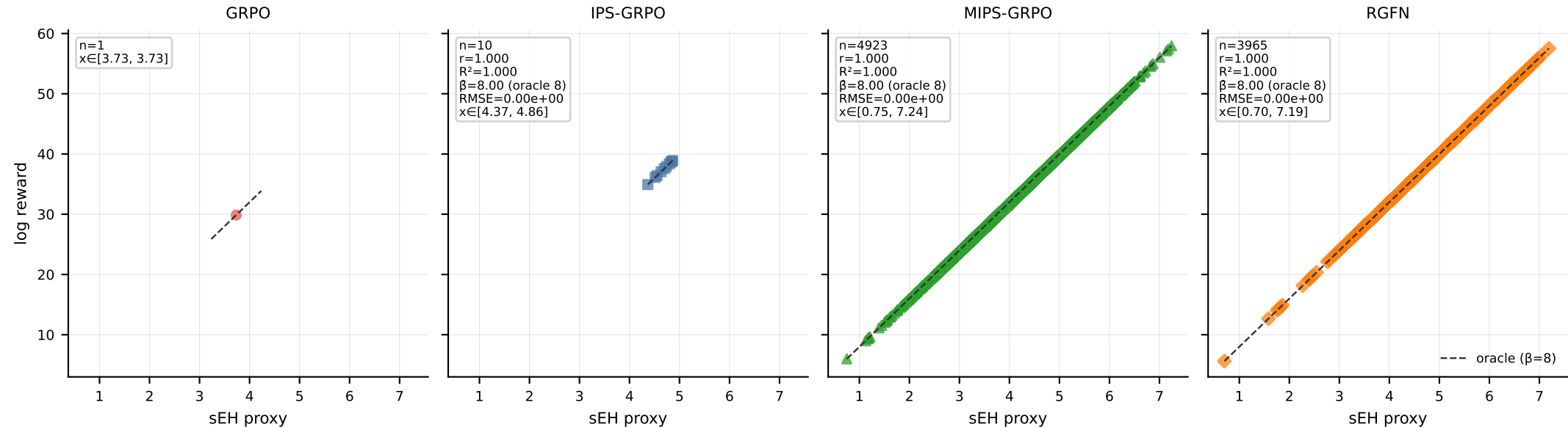
Supplementary: unique-terminal log reward vs proxy (linear oracle)
