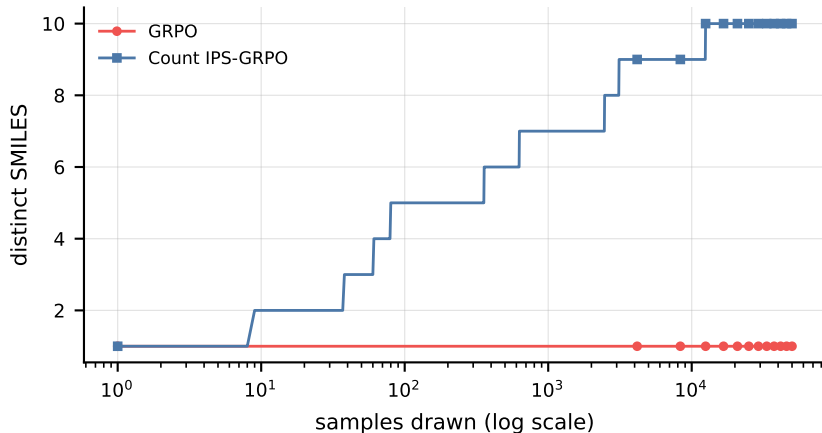
(a) support discovery
