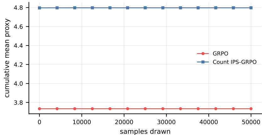
(b) running mean proxy
