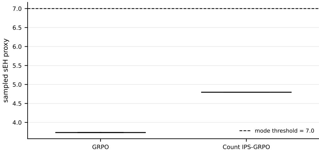
Final-policy sampling @ 2,000 iterations (50,000 samples)
