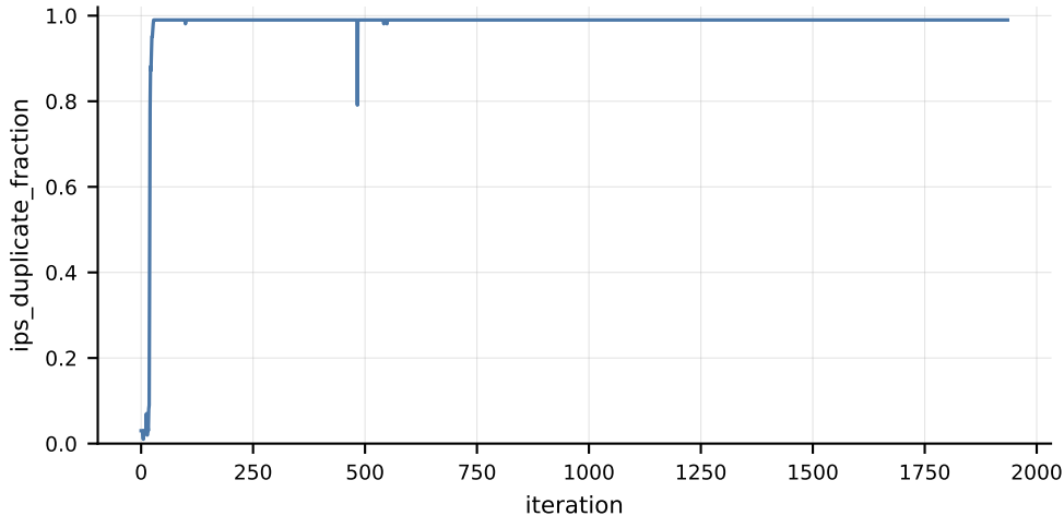
Count IPS-GRPO — duplicate outcome fraction during training
