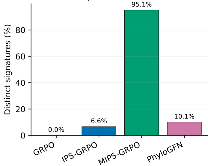
Non-repetition in 1M draws
