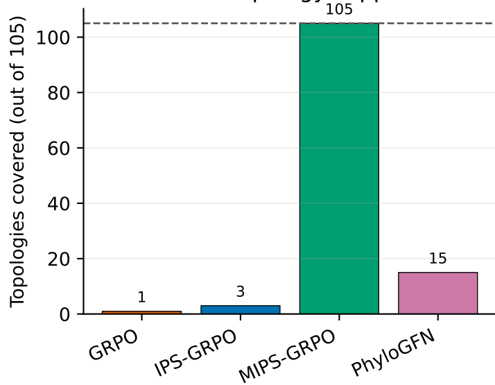
Exact topology support
