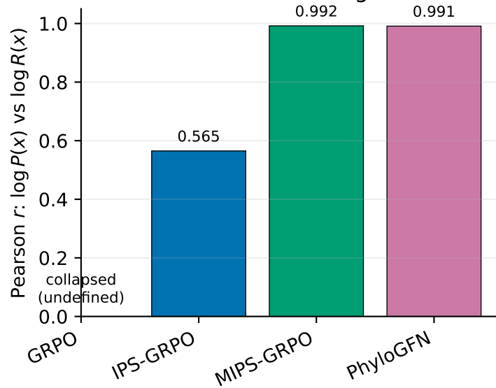
Pathwise reward alignment
