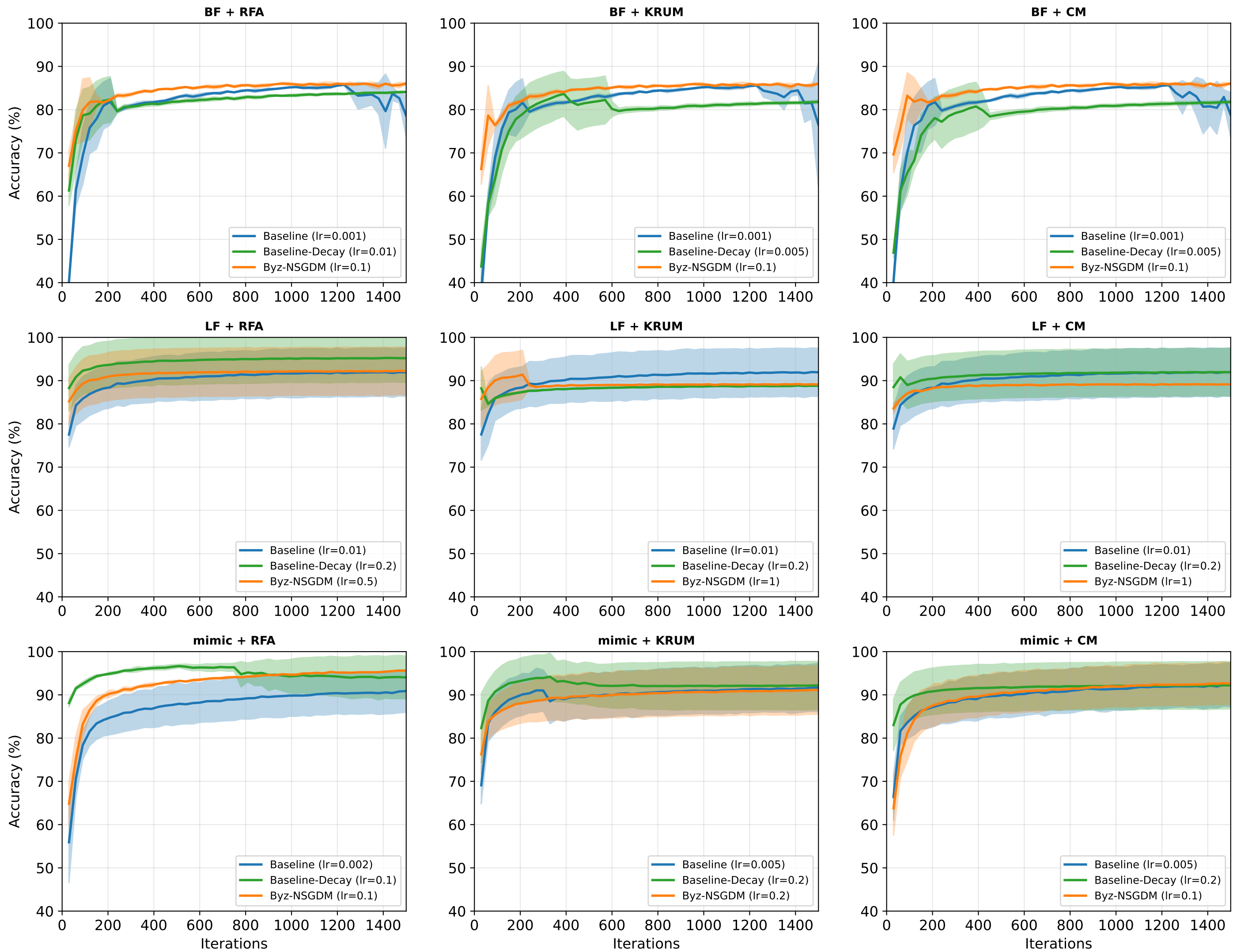
Baseline vs Baseline-Decay vs Byz-NSGDM (best LR per setup)
