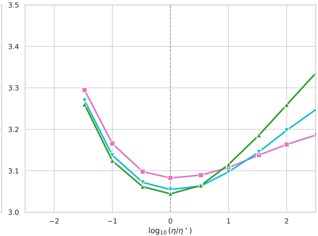
160M Chinchilla
