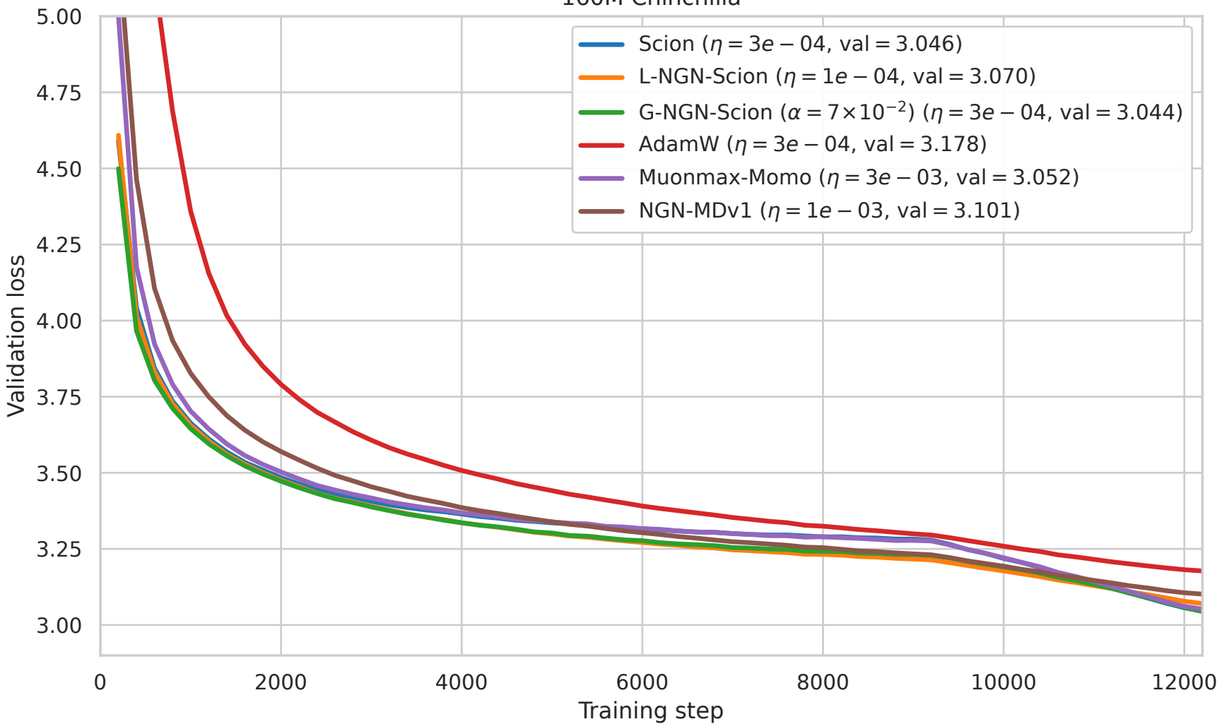
160M Chinchilla
