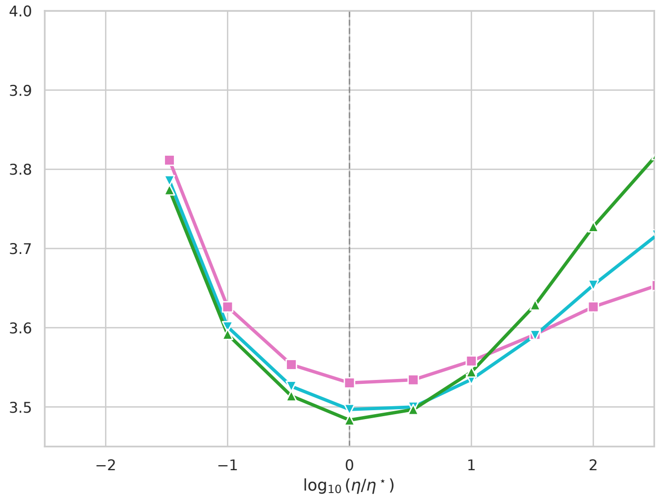
70M Chinchilla
