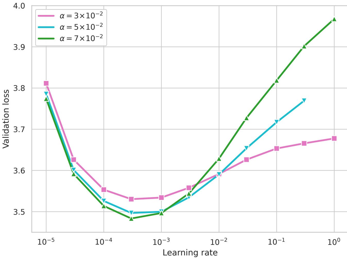
70M Chinchilla
