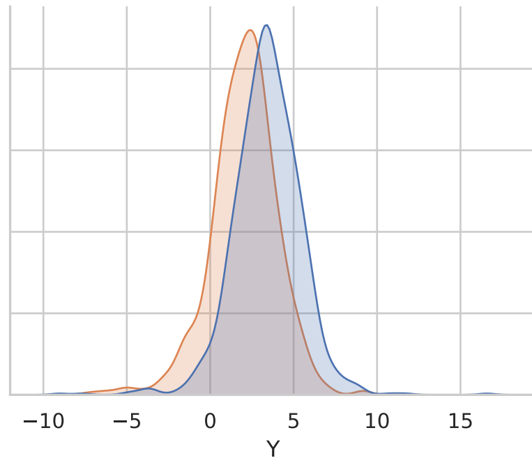
Modele generateur = Modele 2
