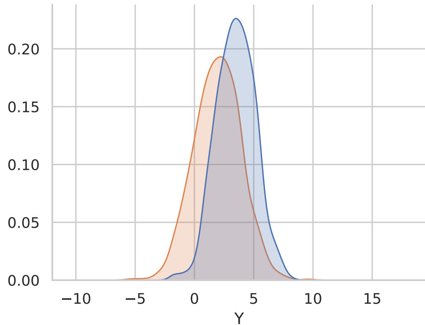
Modele generateur = Modele 1
