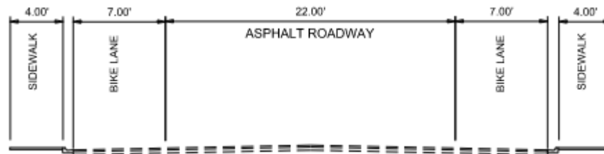
Figure 6: Constitution Avenue from Manana Avenue to Washington Street - Existing Typical Section
