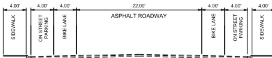
Figure 4: Washington Street from Joe Dan Place to Indian School Road - Existing Typical Section
