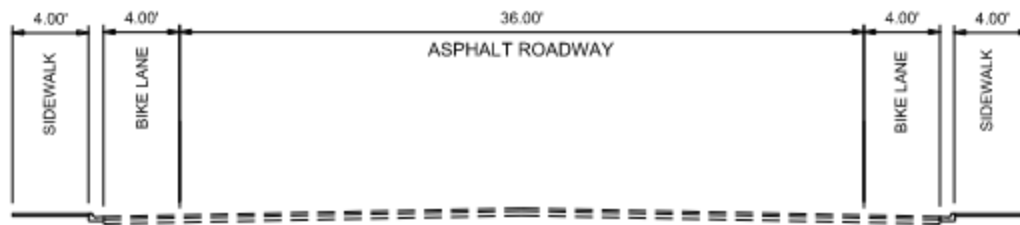
Figure 5: Constitution Avenue from Carlisle Avenue to Manana Avenue - Existing Typical Section
