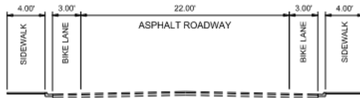
Figure 2: Washington Street from Marble Avenue to Constitution Avenue - Existing Typical Section
