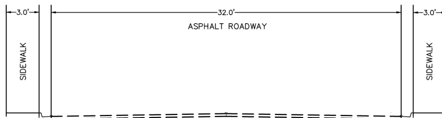
Figure 13: Solano Drive - Existing Typical Section from Mackland Avenue to Lomas Boulevard
