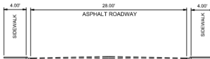
Figure 7: Morningside Drive - Existing Typical Section
