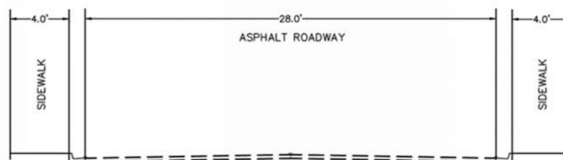
Figure 12: Solano Drive - Existing Typical Section from Indian School Road to Mackland Avenue
