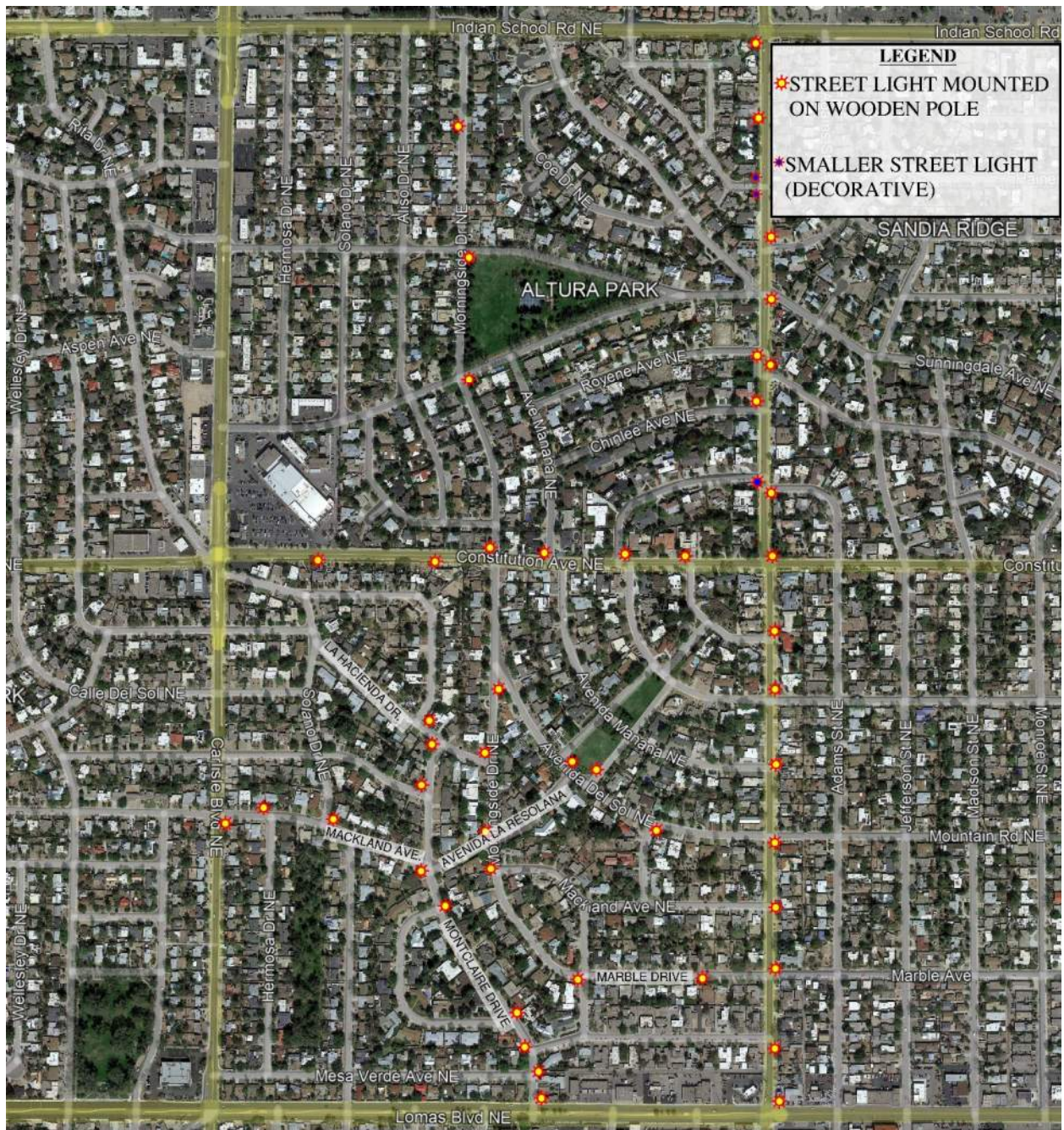
Figure 20: Street Lighting Locations
