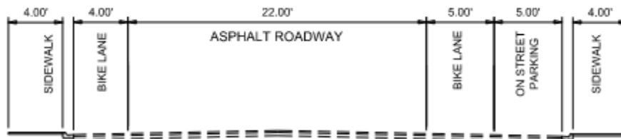
Figure 3: Washington Street from Constitution Avenue to Joe Dan Place - Existing Typical Section
