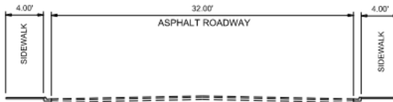
Figure 10: Montclair Drive - Existing Typical Section
