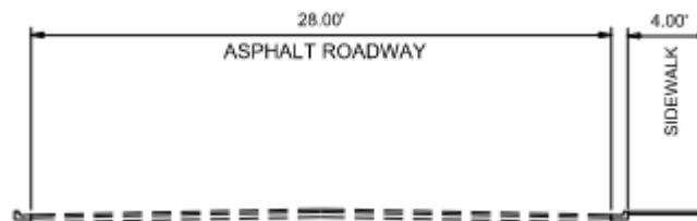
Figure 8: Aspen Avenue - Existing Typical Section
