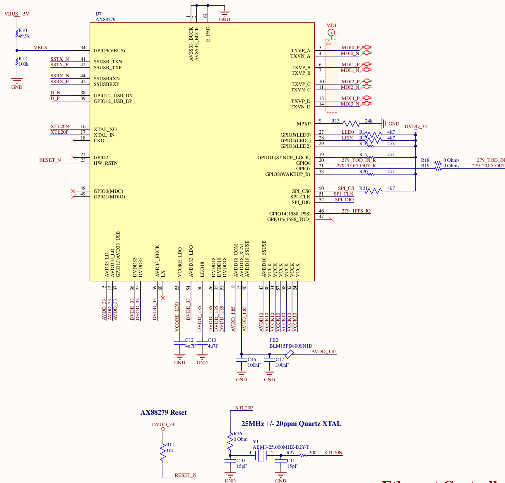
Ethernet Controller
