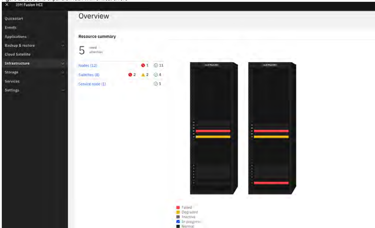
Figure 2. Base and expansion rack with critical errors
