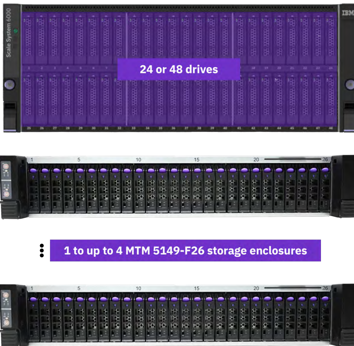
Figure 10. Hybrid configuration with 48 or 24 drives installed and one or more MTM 5149-F26 storage enclosures
