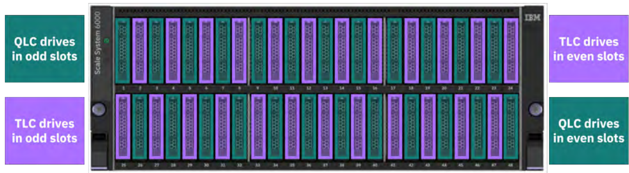
Figure 12. Fully populated IBM Storage Scale System 6000 with 24 QLC drives and 24 TLC drives
