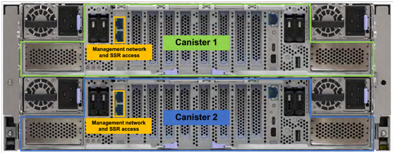
Figure 30. SSR and management access ports in the IBM Storage Scale System 6000
