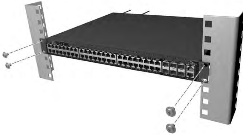
Figure 139. Securing the MTM 5149-S54 switch to the rack
