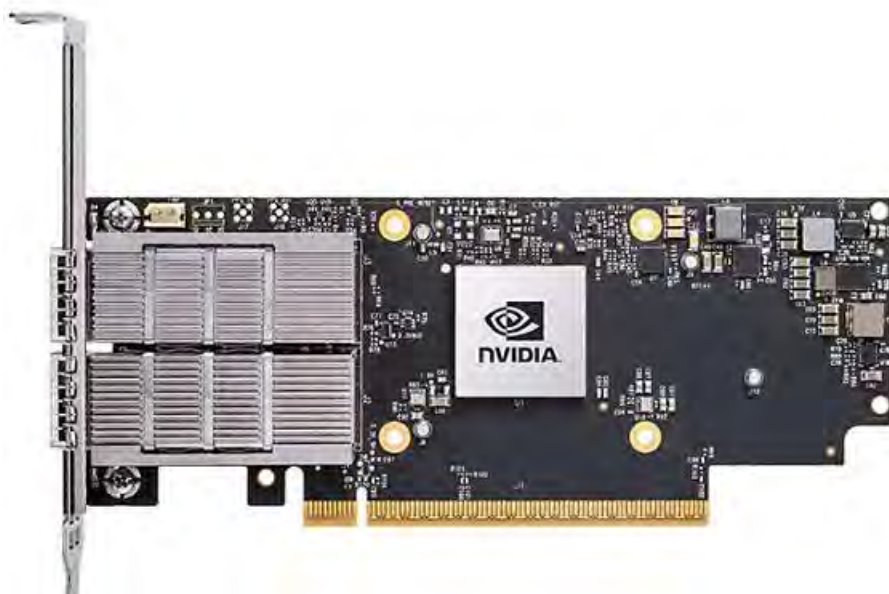
Figure 52. 2-port HDR 200 Gb InfiniBand ConnectX-7 adapter (FC AJQS)
