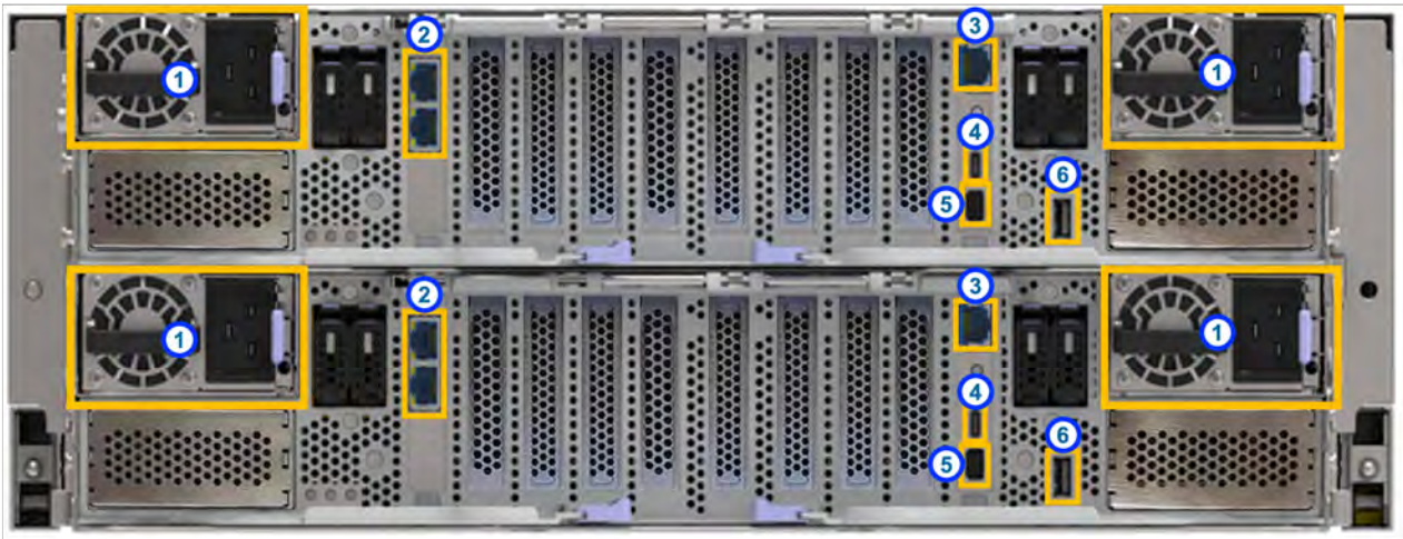
Figure 27. Orientation of ports on IBM Storage Scale System 6000
