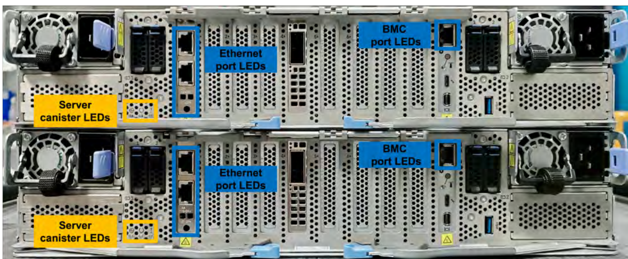
Figure 46. IBM Storage Scale System 6000 server canister LEDs
