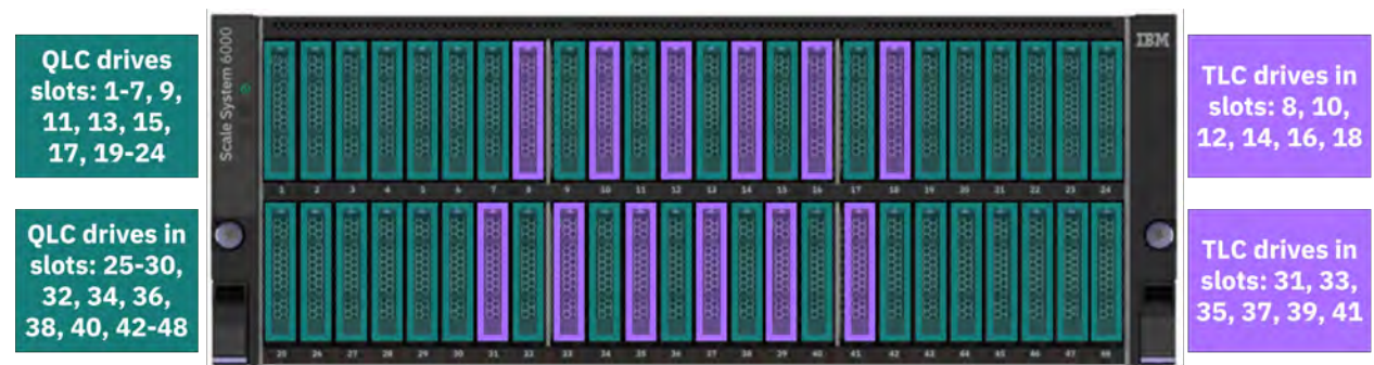
Figure 13. Fully populated IBM Storage Scale System 6000 with 36 QLC drives and 12 TLC drives
