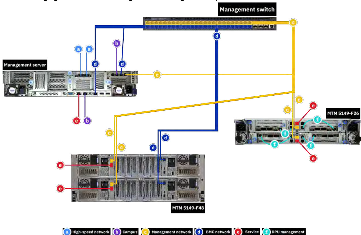
Figure 31. BMC and management network connections
