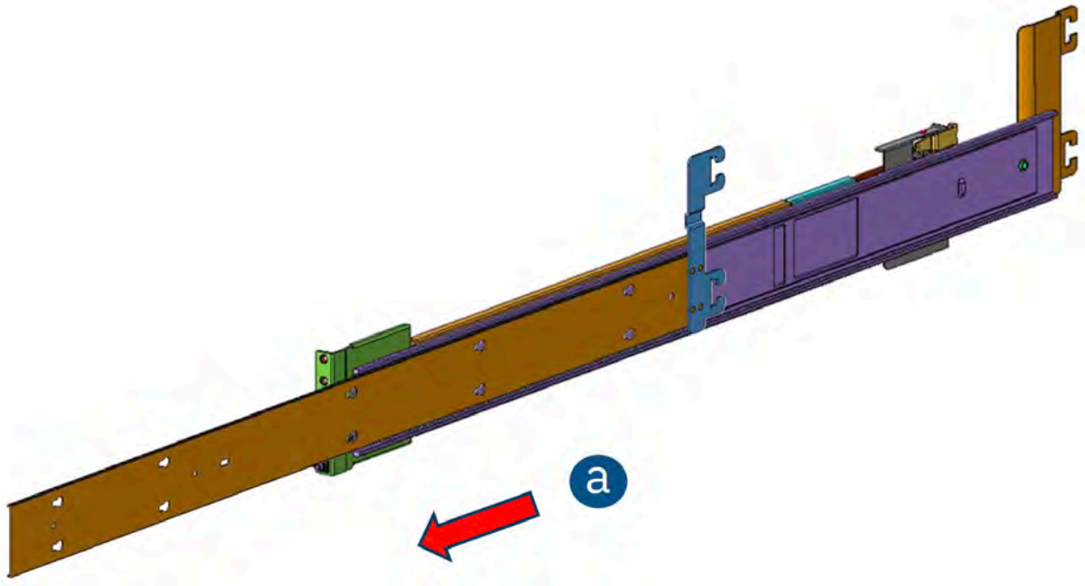
Figure 32. Pulling the inner rail
