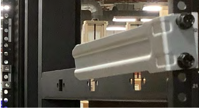
Figure 106. Placing a rack mounting blade on a right rack post
