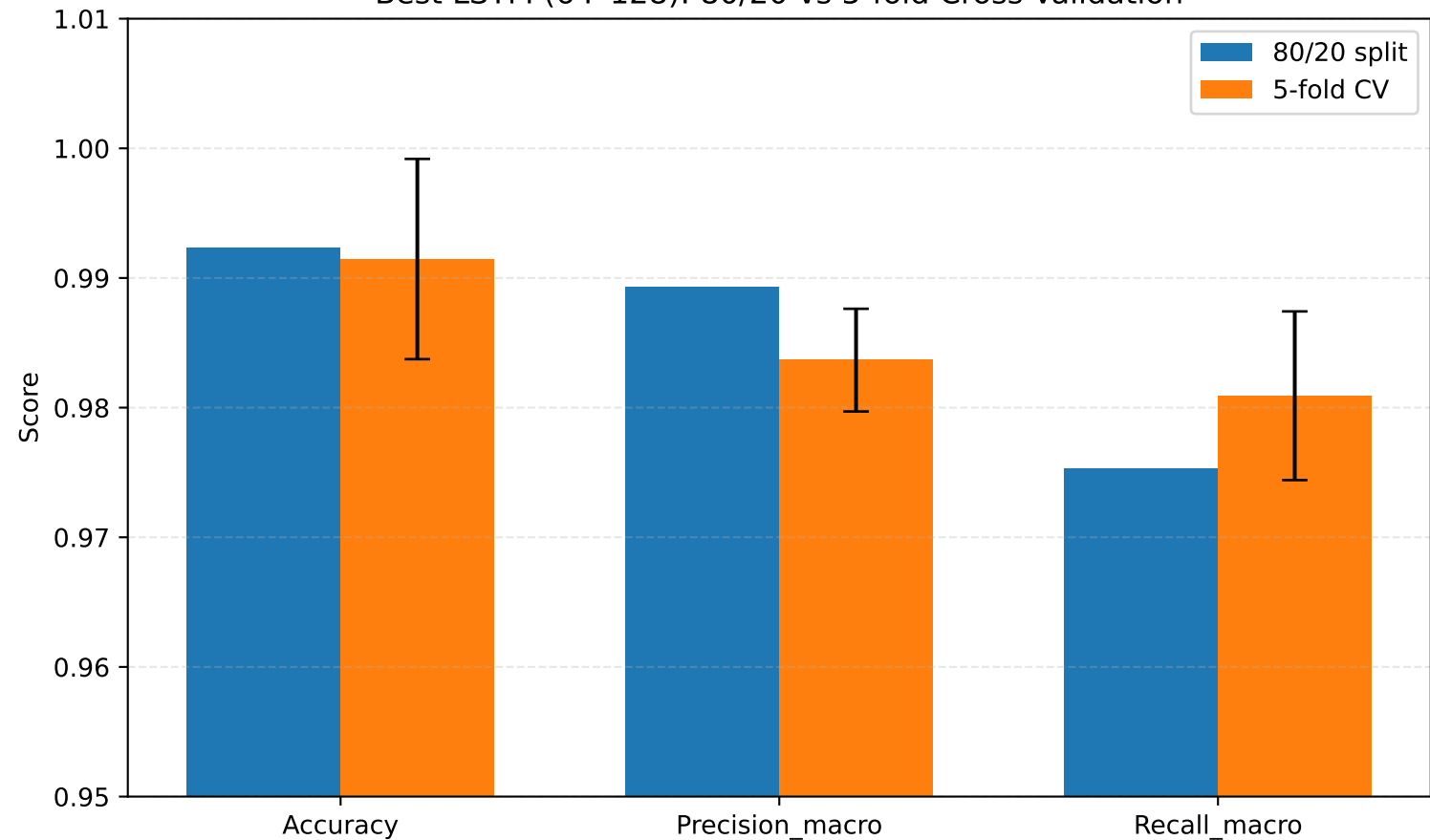
Best LSTM (64-128): 80/20 vs 5-fold Cross-Validation
