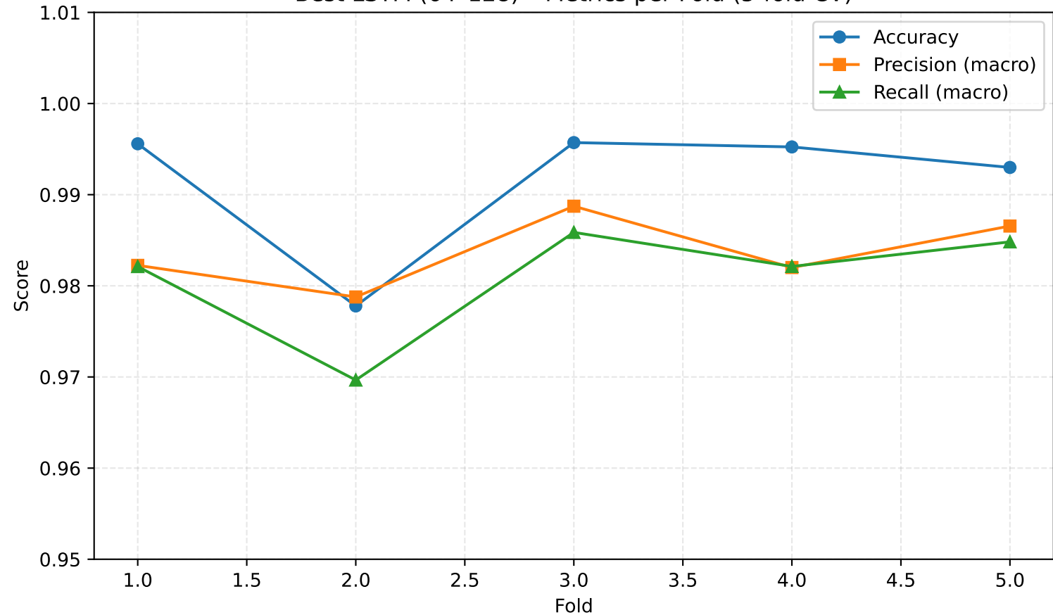
Best LSTM (64-128) - Metrics per Fold (5-fold CV)
