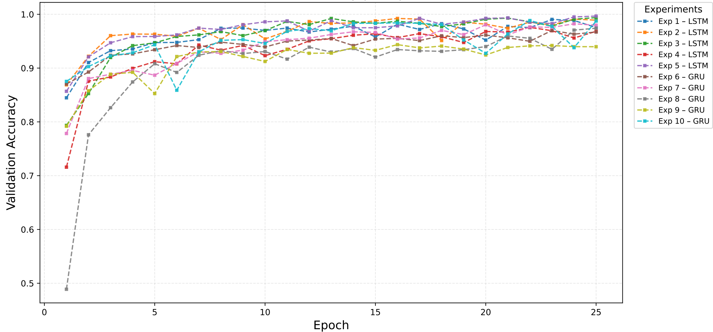
Validation Accuracy per Epoch
