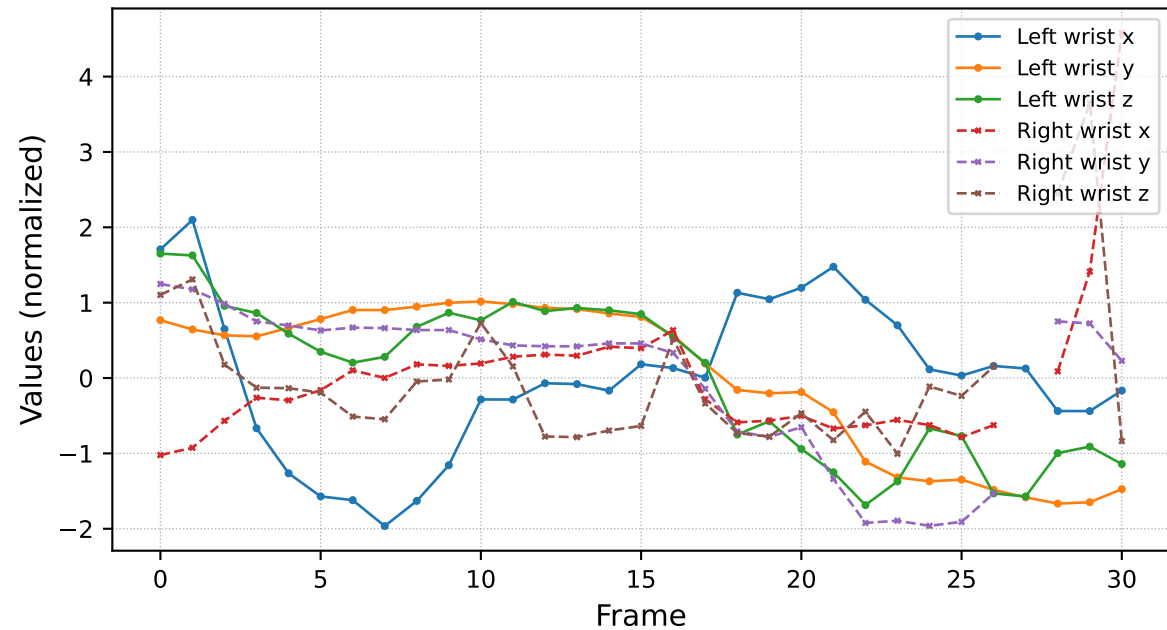
Wrist Landmark Dynamics for the Sign "Doctor" (up to frame 30)
