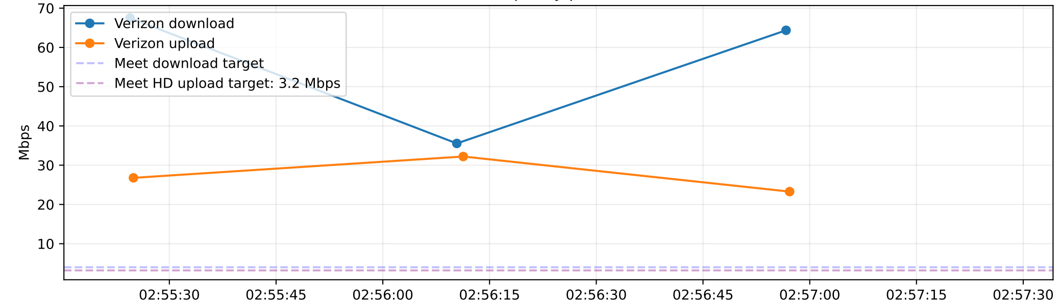
Capacity probes
