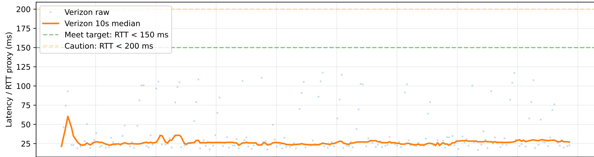
Latency
