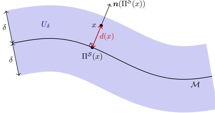
Figure I.1. Strip U_\delta around the hypersurface \mathcal{S} and normal coordinates x = \Pi^\mathcal{S}(x) + d(x) \nu(\Pi^\mathcal{S}(x))
