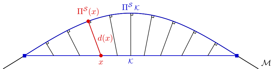
Figure I.16. A curved simplex \Pi^S \mathcal{K} is parametrized over a planar one. Orthogonal projection onto the smooth surface \mathcal{M}
