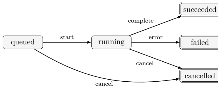
Figure .1. Agent-run lifecycle state machine (FR-AE-01, EC-FC-01). Double-bordered states are terminal.
