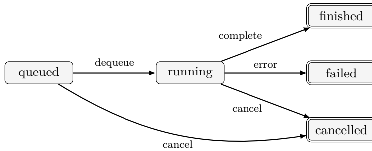
Figure .2. Job lifecycle state machine (FR-JB-02, EC-FC-07). Cancellation is cooperative: the worker checks a cancellation flag between steps.
