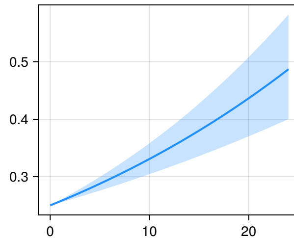
Embedded NSM — posterior predictive (mean + 90% band)
