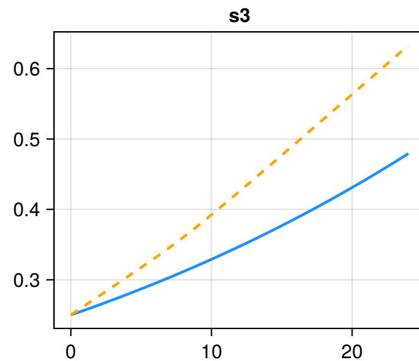
Embedded NSM vs gLV-residual PINN (Option 1) — same data, same solver
