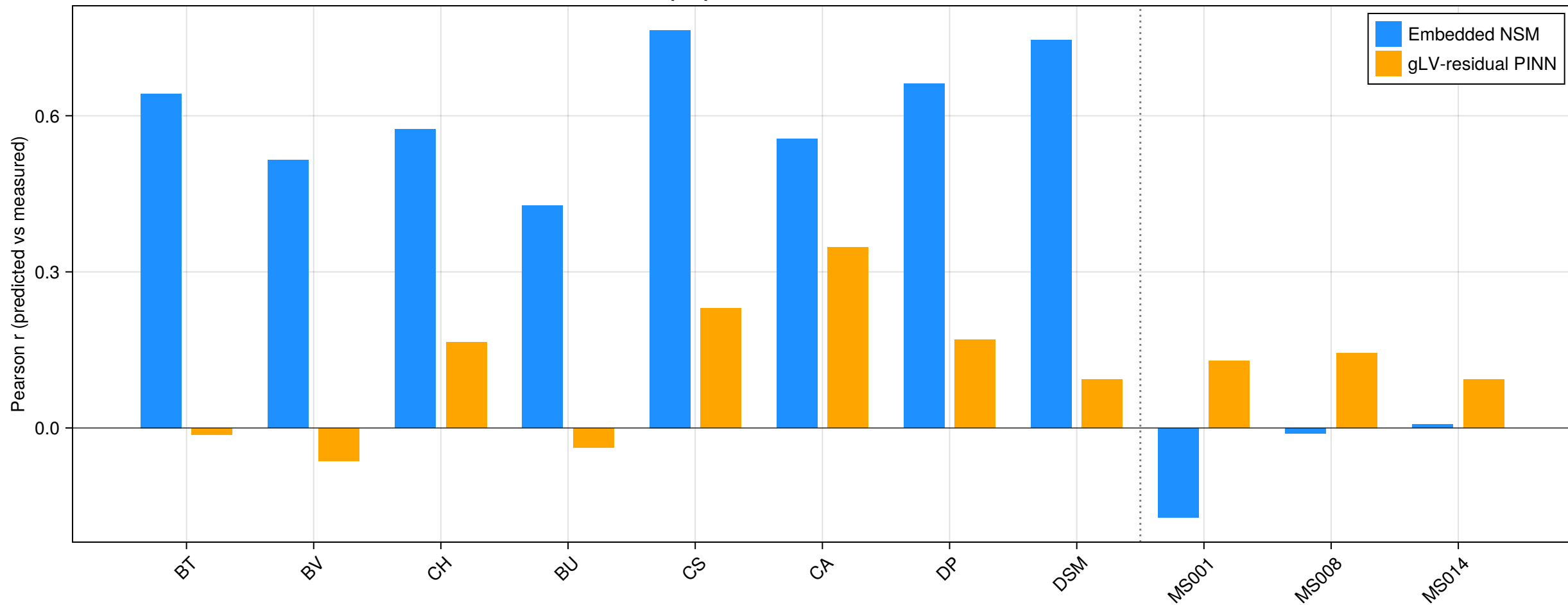
Per-output prediction correlation on held-out Cdiff
