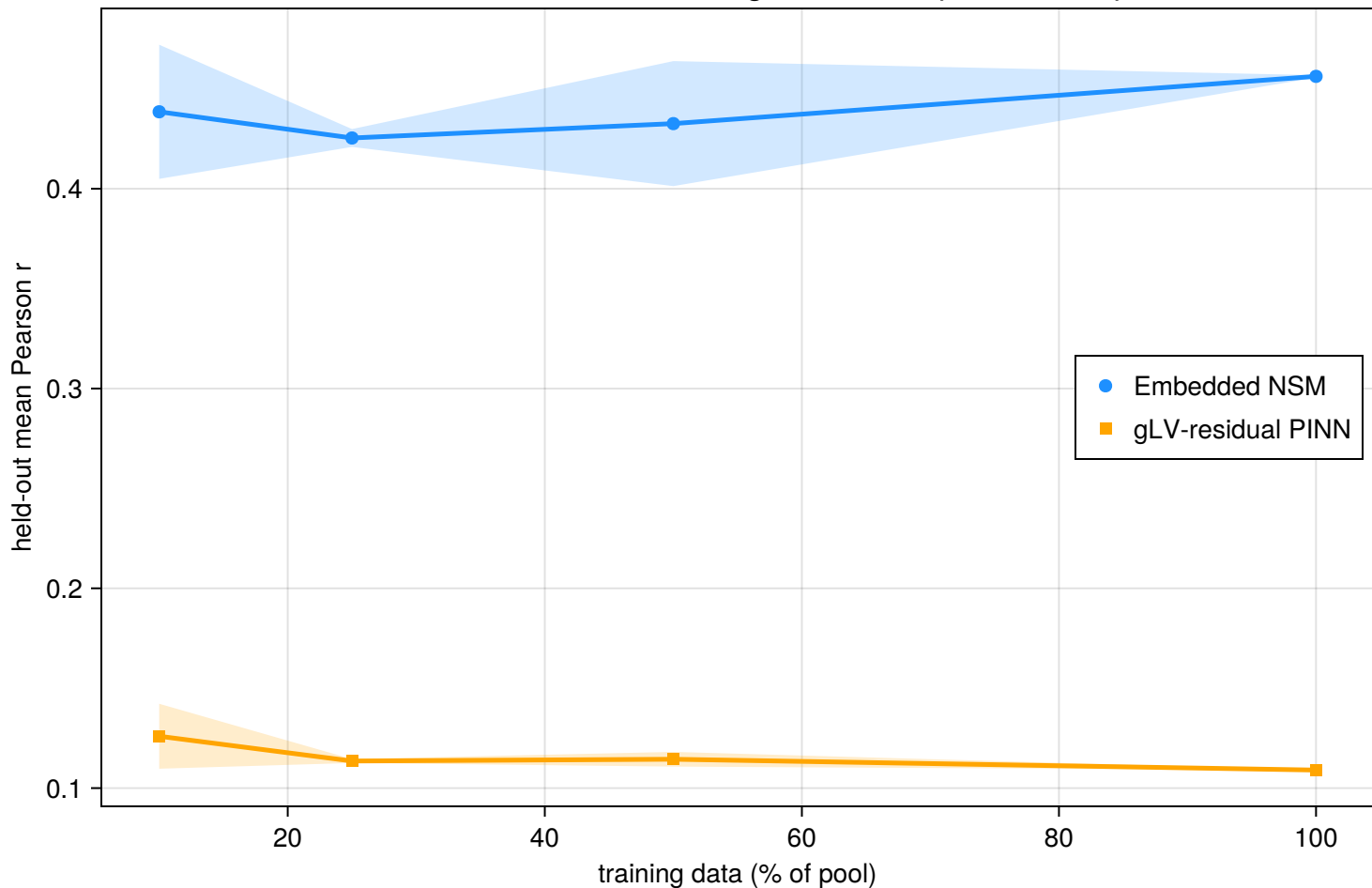
Prediction correlation vs training-data amount (Cdiff held-out)
