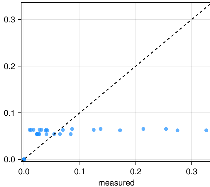
Embedded CRM NSM — Sulfide r=0.5
