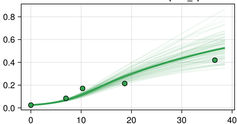
NSM — held-out co-culture (Pair_1)
