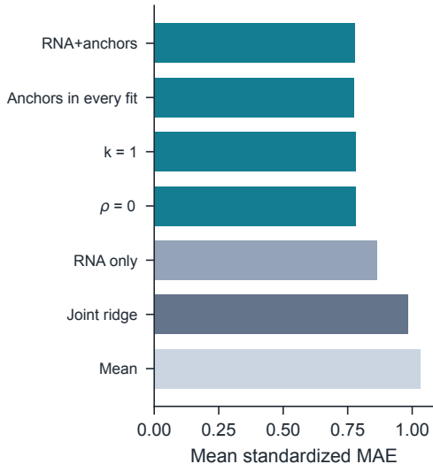
b What the fit uses
