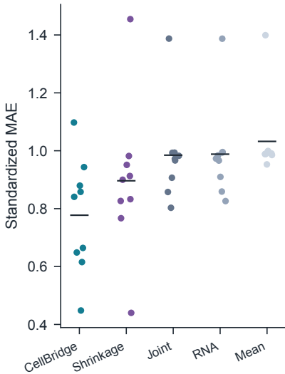
a Nine development tasks
