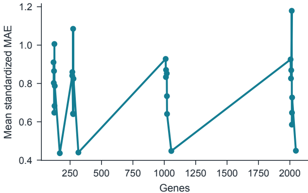
Gene count, reduced grid
