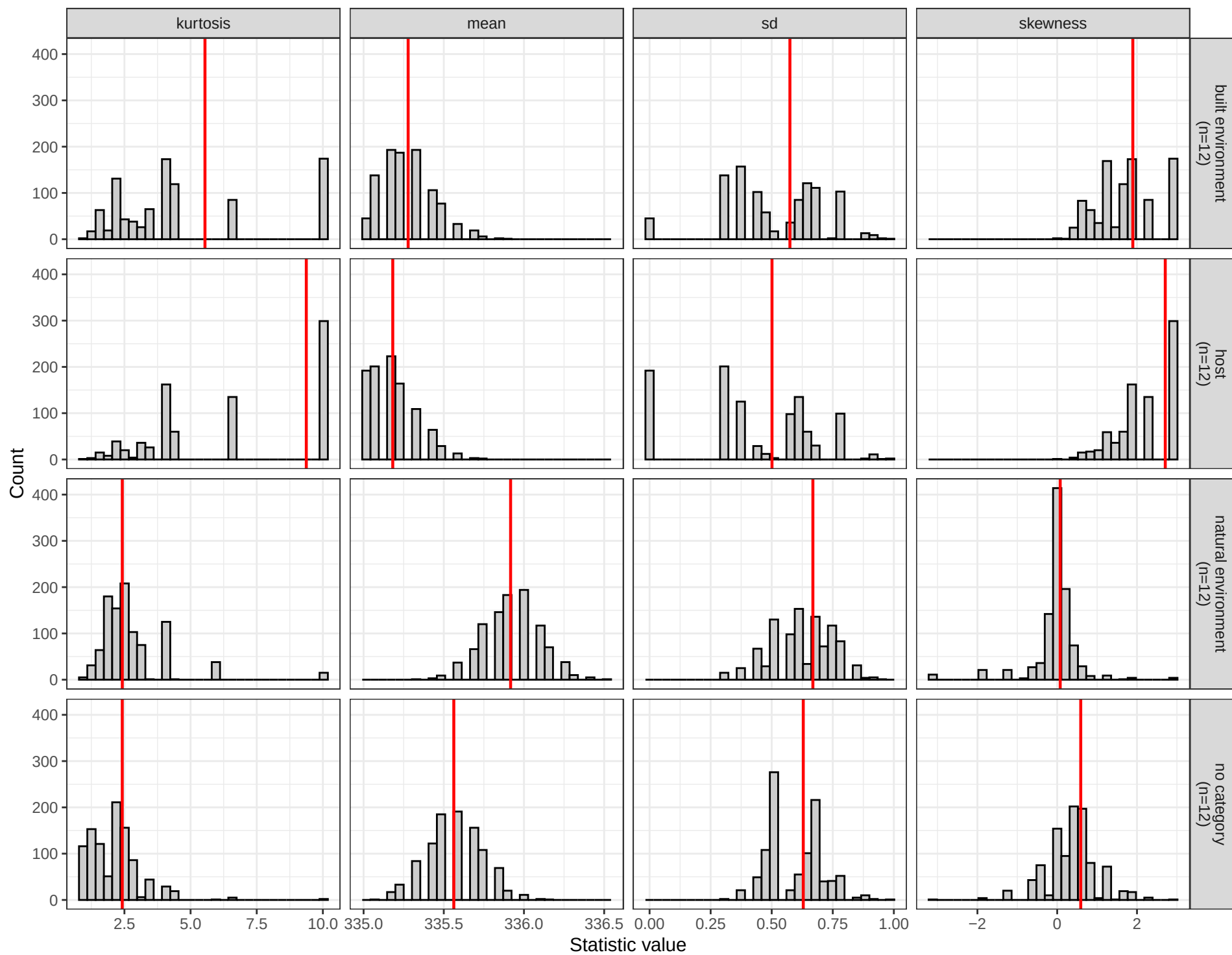
Bootstrapped distributions of sequence_length statistics by category
