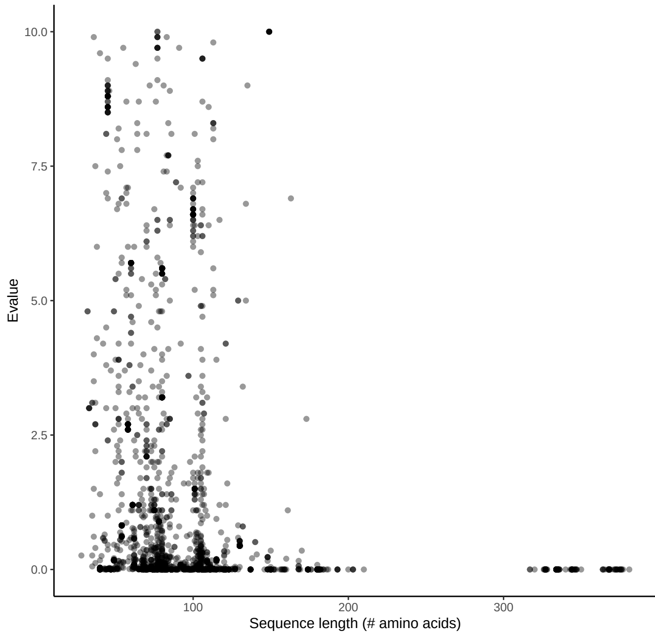
Sequence length vs evalue plot (n=3223 BLAST hits)
