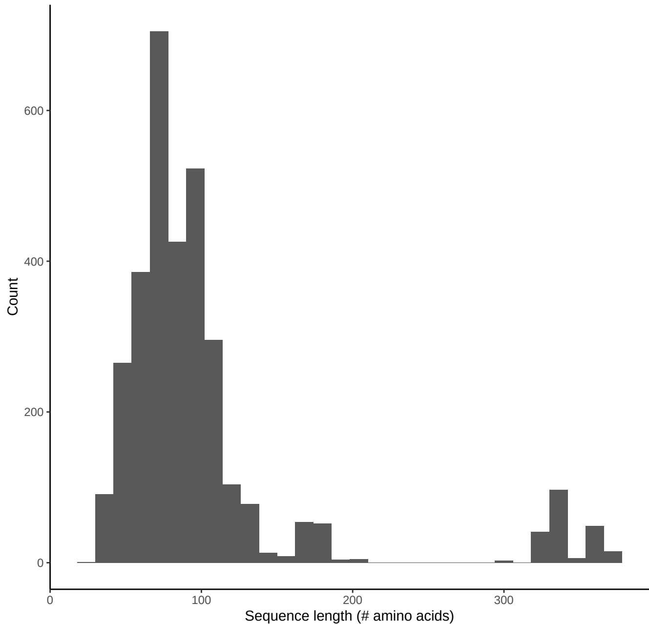
Sequence length frequencies, gaps removed (n=3223 BLAST hits)
