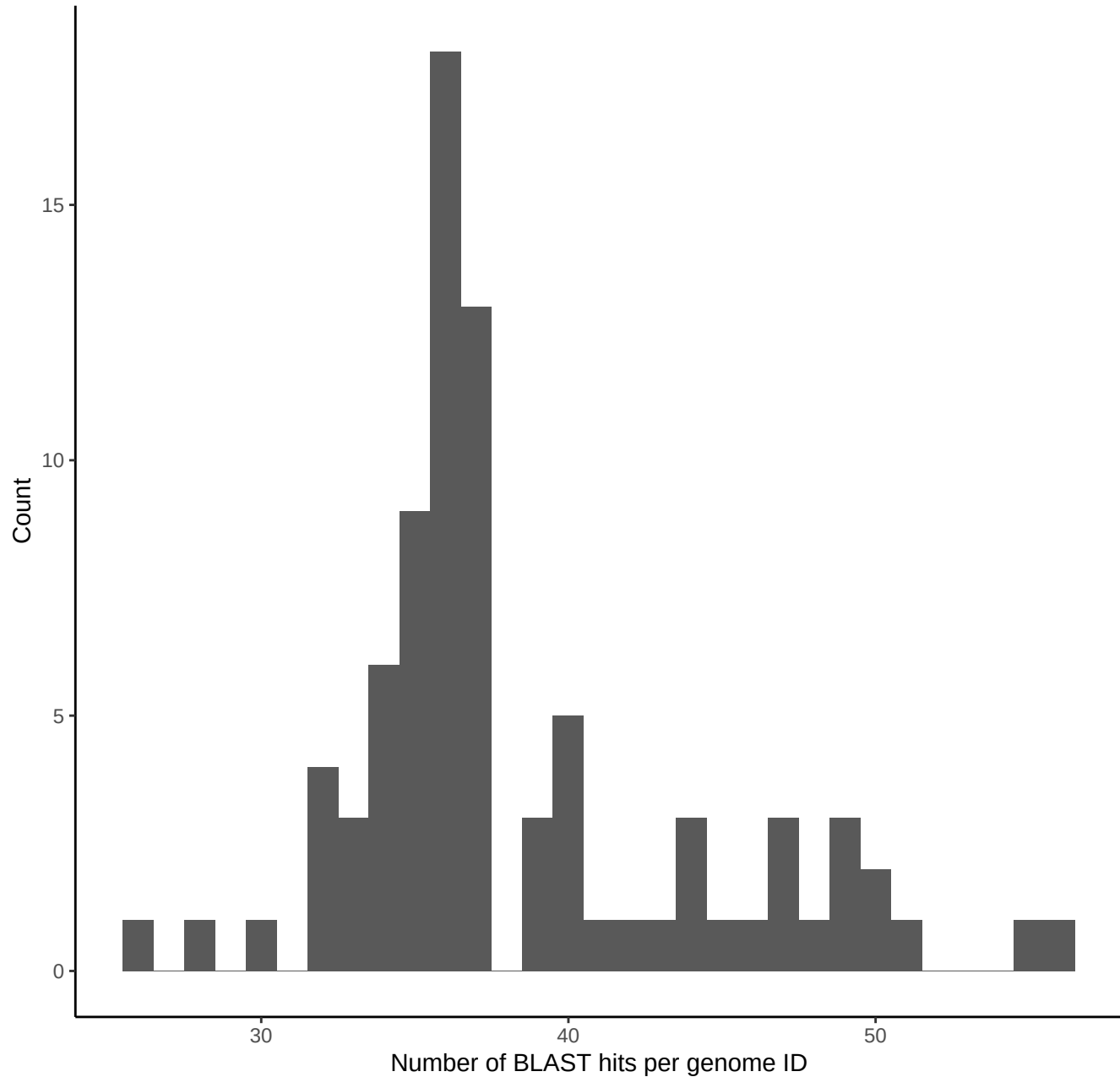
Genome ID frequencies (n=3223 BLAST hits)
