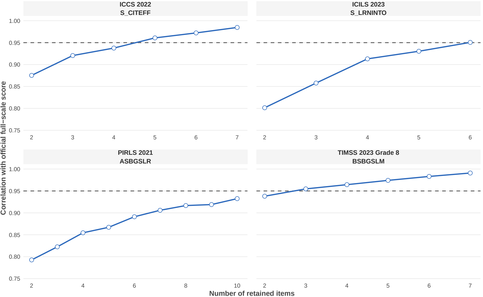
Figure S3. Recovery of the full scale as item count decreases
