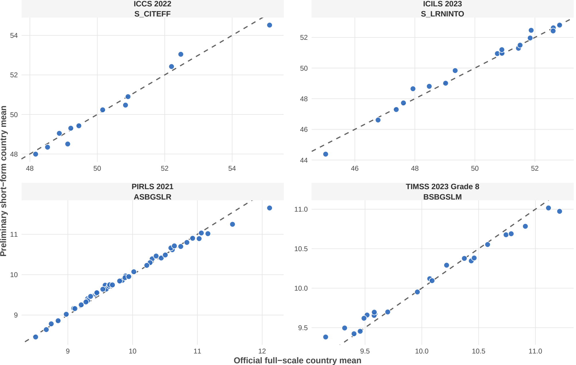
Figure S4. Country means from preliminary short forms versus full scales
