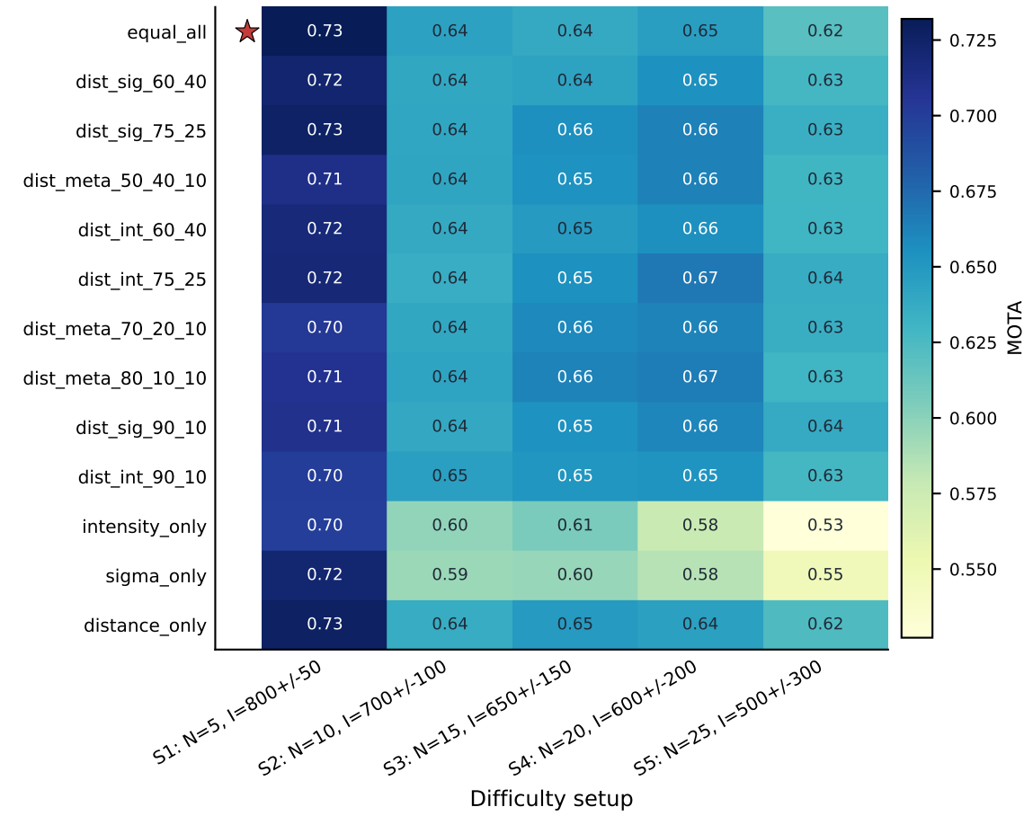
Peak-to-peak MOTA
