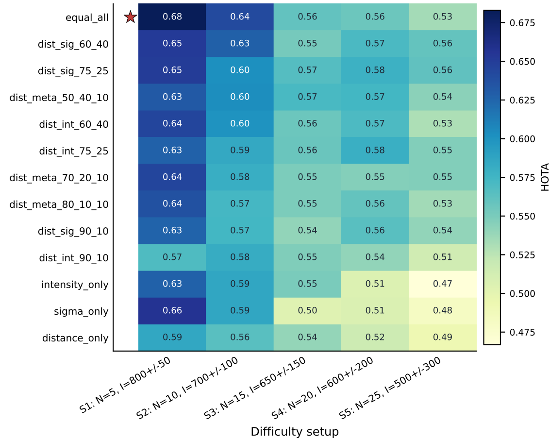
Peak-to-peak HOTA
